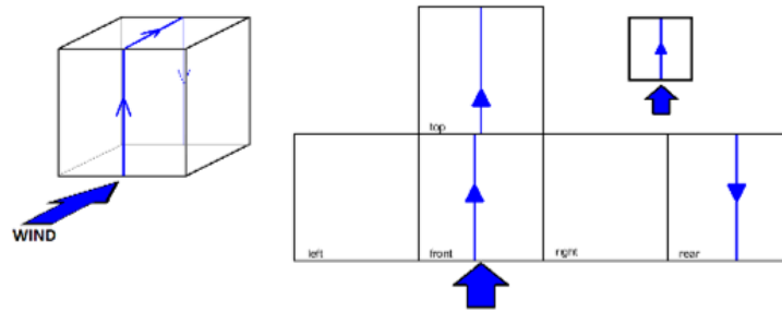
Figure 10. Path along the cube centre line, see also Figure 4 for the specific pressure taps.
