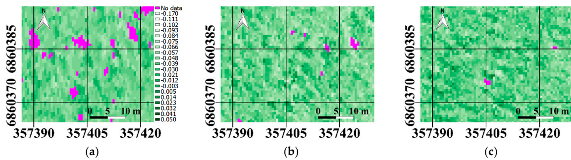
Figure 5. Spatial variation of the canopy PRI for \beta = 19^\circ (a); \beta = 55^\circ (b); and \beta = 76^\circ (c). Purple pixels were masked out ( \text{NDVI} < 0.8 ). The color scale is the same for all three rasters.
