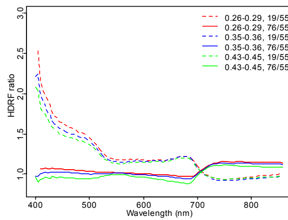
Figure 8. Ratio of Scots pine TOC spectral reflectance between sunlit fractions for three scatter angles ( \beta = 19^\circ, 55^\circ, \text{ and } 76^\circ ).
