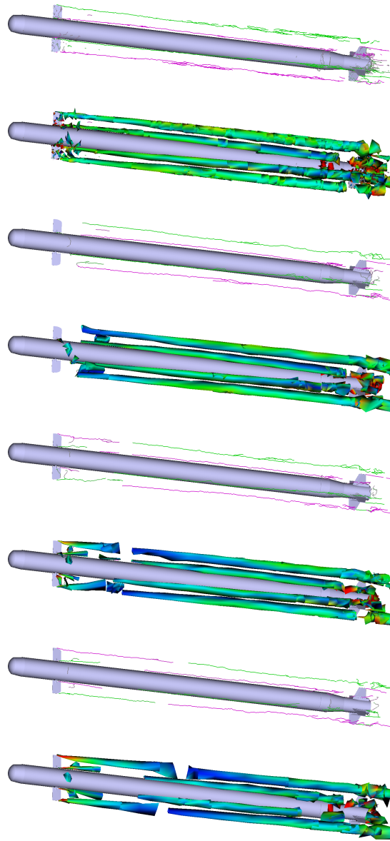
Fig. 1.6. Vortex core lines and extent for spinning missile with dithering canards for time steps t=726, 728, 730, and 732 (top to bottom). Purple indicates a left handed rotation while green indicates a right handed rotation. Alternate images show vortex extent with surface colored by the local tangential velocity. The scale on the non-dimensional tangential velocity is blue (0) to red (0.189).
