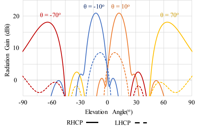
Fig. 3. Spiral antenna array elevation scanning range at \phi = 210^\circ .
