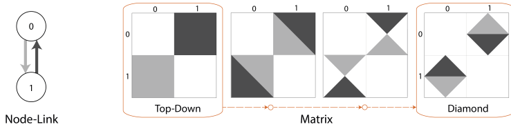
Fig. 7. The evolution of the design for comparing edges of opposite directions. Intermediate design options created ambiguities and visual artefacts because of adjacent neighbouring edges. In the final design (diamond mode), only the (top and bottom) triangles that encode the opposite directions (in and out respectively) appear adjacent.
