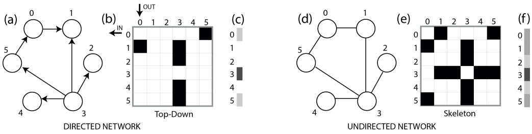
Fig. 5. Directed versus undirected node-link and matrix representations. (a) Node-link representation of a directed network. (b) The same directed network as encoded in top-down mode. Rows encode incoming edges and columns outgoing edges resulting in an adjacency matrix that is not symmetric. (c) The out-degree of each node as encoded using opacity in a summary column. (d) Node-link representation of an undirected network. (e) The undirected network shown in skeleton-mode resulting in a symmetric adjacency matrix (MultiPiles visualisation method). (f) The degree of each node as encoded using opacity in a summary column.
