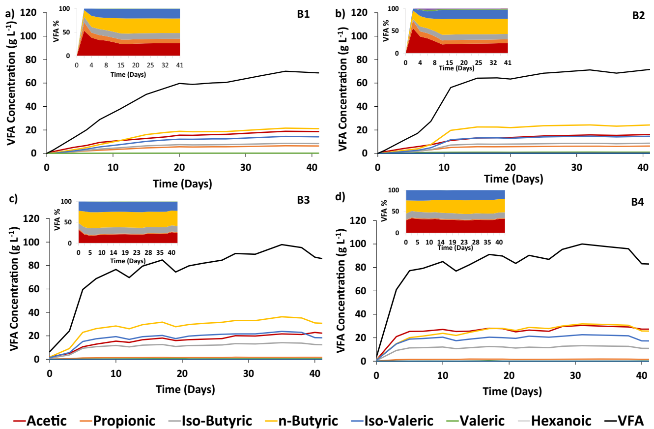
Fig. 1 VFA profiles over the course of the 1-L batch experiment. a Reactor B1. b Reactor B2. c Reactor B3. d Reactor B4. The embedded images correspond to the VFA composition for each reactor
