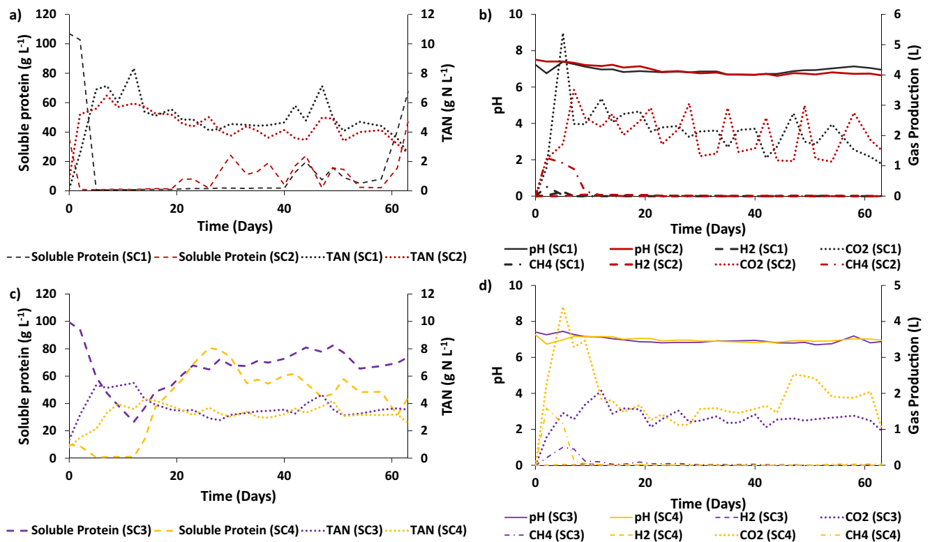
Fig. 5 Soluble protein, TAN, gas production and pH of semi-continuous experiment. a Soluble protein and TAN concentrations of reactors SC1 and SC2. b Gas production and pH of reactors SC1 and SC2; gas production data represent the CO 2 , H 2 and CH 4 produced during each of SC2 feeding cycle. c Soluble protein and TAN concentrations of reactors SC3 and SC4. d Gas production and pH of reactors SC3 and SC4; gas production data represent the CO 2 , H 2 and CH 4 produced during each of SC4 feeding cycle
