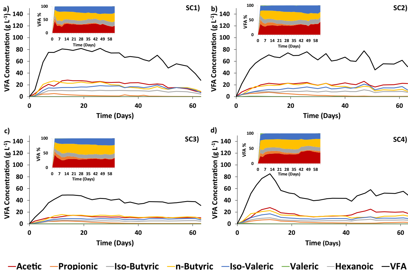
Fig. 4 VFA profiles of the semi-continuous experiment. a Reactor SC1. b Reactor SC2. c Reactor SC3. d Reactor SC4
