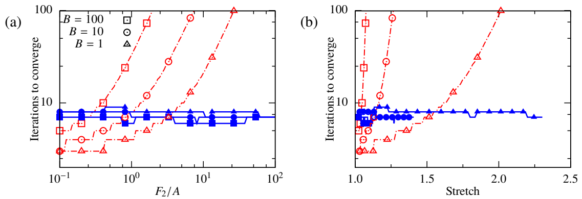
Figure 7: Iterations taken to converge for the 1D extension problem with Veronda-Westmann model using the standard (red dashed line and open symbols) and log formulation (blue solid line and filled symbols) with F_1/A = 10^{-4} and varying B .
