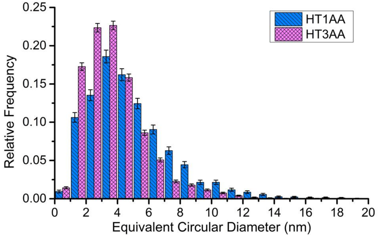
Figure 17 Histograms showing the size distributions of the \beta -NiAl phase precipitates after heat treatment HT1AA and HT3AA.
