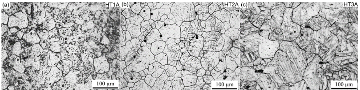
Figure 7 Optical micrographs shows the prior austenite grain structures after austenisation heat treatments in (a) HT1A, (b) HT2A and (c) HT3A.
