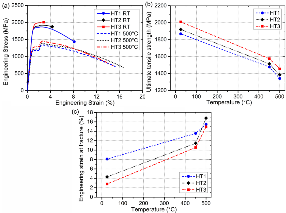
Figure 2 (a) Tensile stress-strain curves for the different heat-treatments at room temperature and 500 °C; changes of, (b) the ultimate tensile strength, and (c) the engineering strain to fracture, for the different heat-treatments at different testing temperatures.
