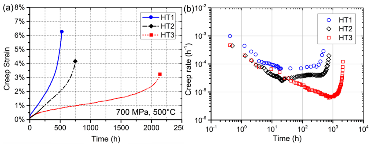
Figure 5 (a) Creep strain-time curves and (b) creep rate-time plots for the steel subjected to three different heat-treatments. The testing condition used is a load of 700 MPa at 500 °C.
