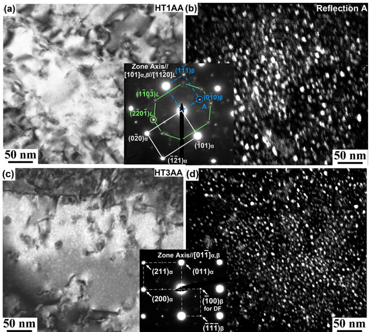
Figure 15 (a) TEM BF micrograph after HT1AA with SADP in insertion showing ferrite, \beta -NiAl superlattice and Laves phase reflections; (b) DF image of the same area of (a) using the \beta -NiAl (0\bar{1}0)_\beta superlattice reflection labelled as A in the SADP. (c) BF micrograph after HT3AA with SADP in insertion, (d) DF image of the same area of (c) using the \beta -NiAl (\bar{1}00)_\beta superlattice reflection.
