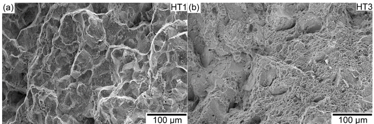
Figure 6 Fracture surfaces of creep tested (700 MPa at 500 °C) samples after (a) HT1 and (b) HT3.
