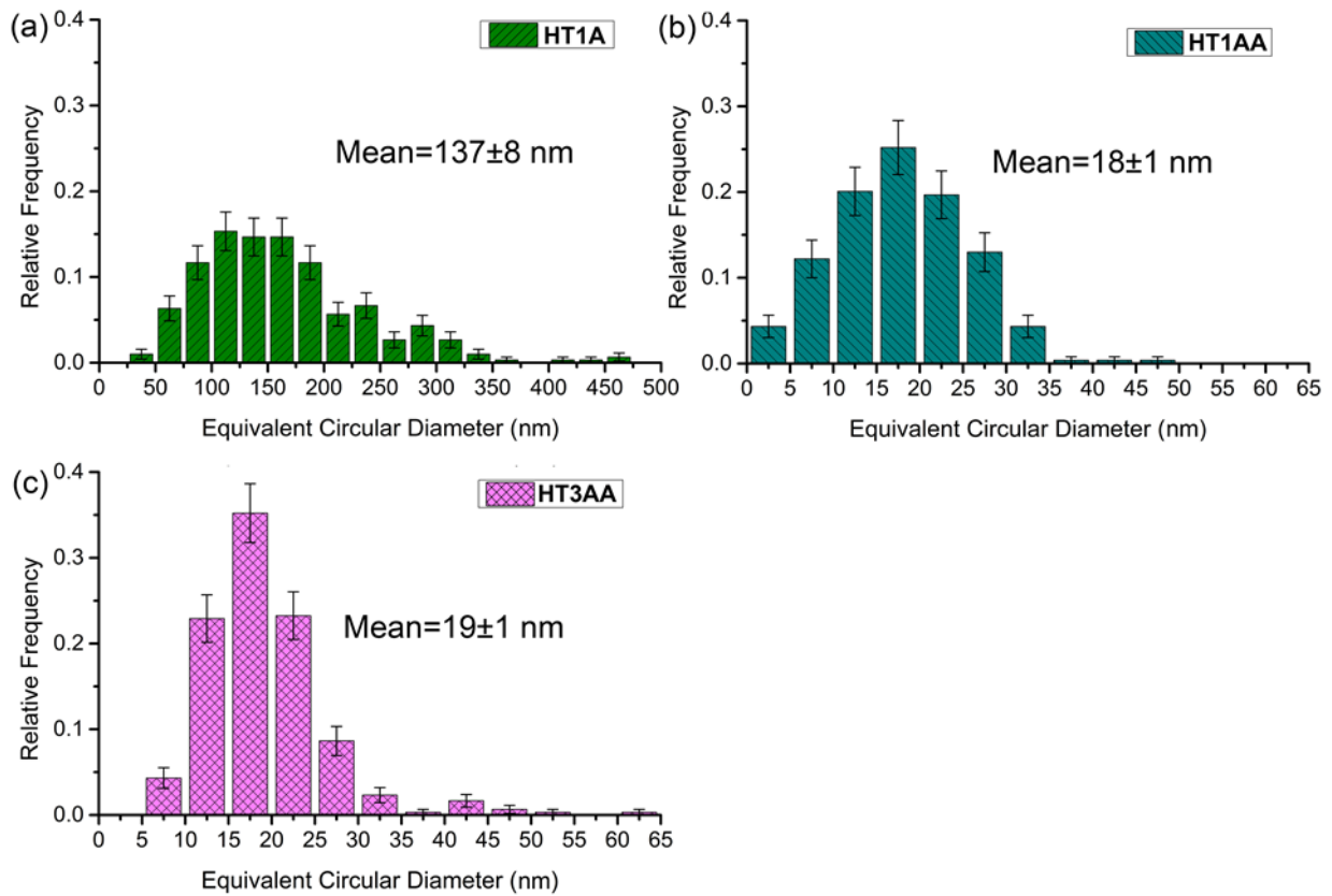
Figure 14 Histograms showing the size distributions of the Laves phase precipitates for (a) Primary Laves formed after austenisation in HT1, (b) secondary Laves formed after ageing in HT1 and (c) the secondary Laves formed after ageing in HT3.
