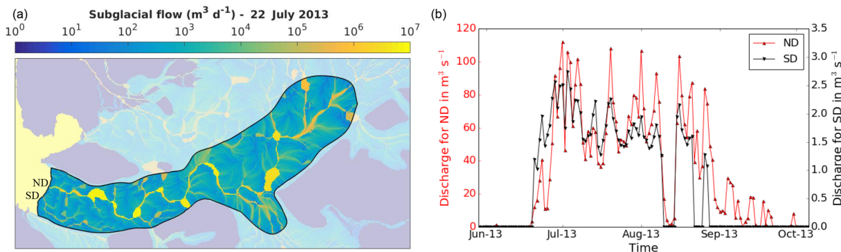
Figure 6. (a) Subglacial flow following the hydraulic potential surface (in \text{m}^3 \text{d}^{-1} ) in logarithmic scale on 22 July 2013. (b) Daily discharge for the northern and southern discharge (ND and SD respectively) during the melting season (data gaps correspond to no discharge).
