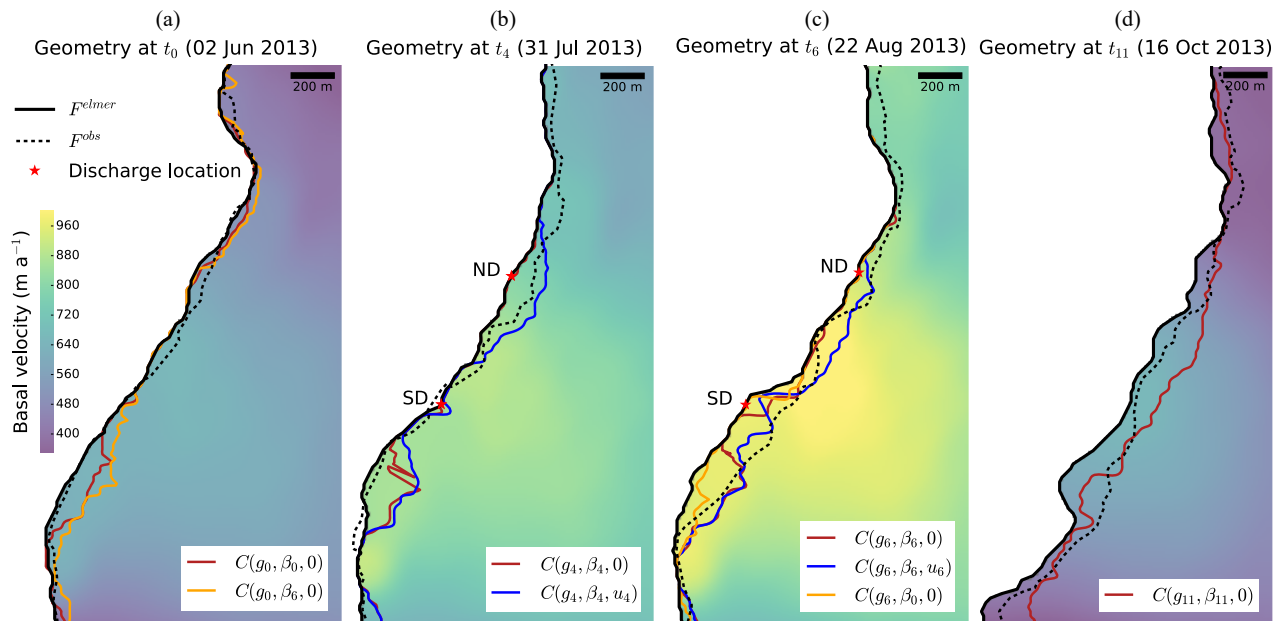
Figure 10. Basal velocity, advanced front before calving modelled with Elmer/Ice, F_i^{\text{elmer}} , at t_i in plain black; observed front after calving, F_i^{\text{obs}} , in dashed black; and calving front modelled with HiDEM, F_i^{\text{hidem}} , given the different configurations summarised in Table 2 for (a) i = 0 , (b) i = 4 , (c) i = 6 , and (d) i = 11 . Discharge locations (for i = 4, 6 ) are marked with a red star.
