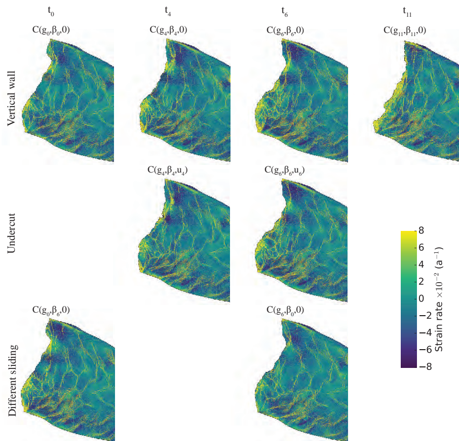
Figure 11. Strain rates modelled with HiDEM for each configuration. Yellow colouring shows the crevasse pattern and is denser close to the front where the difference between each configuration for the four selected iterations can be observed.
