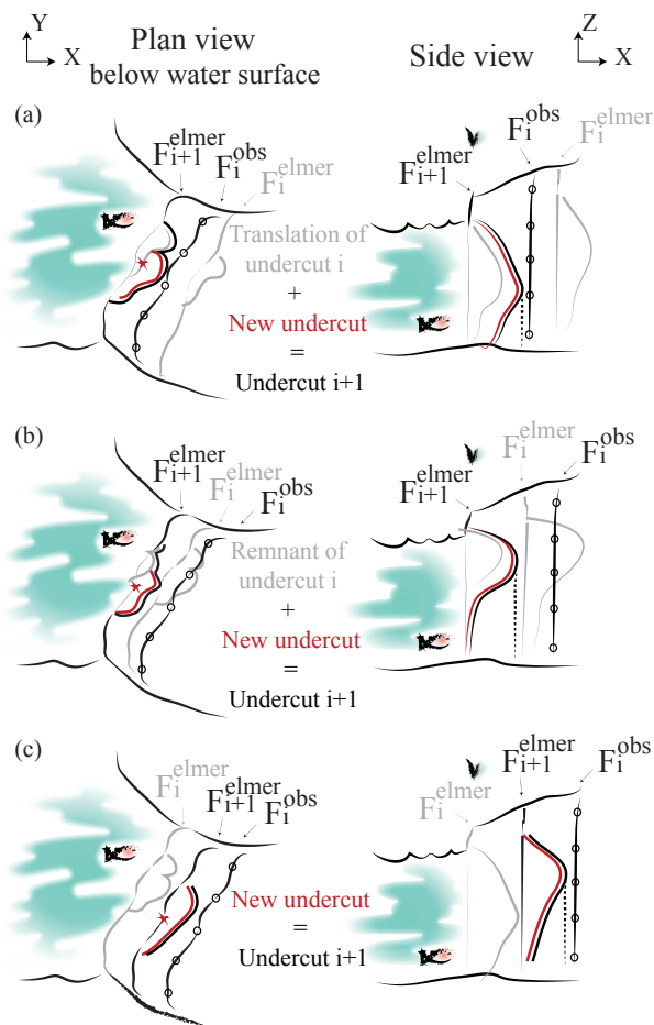
Figure 4. Three cases of undercutting i+1 at t_{i+1} (black line) depending on former undercutting i at t_i (grey line) at z relative to F_i^{\text{obs}}(z=0) (black line with circles) in plan view (left) and side view (right). The red star represents the discharge location. On the side view, the dashed line represents the simplified undercut geometry where the ice foot has been removed, which is given as input to the HiDEM. (a) F_i^{\text{obs}}(z=0) is behind F_{i+1}^{\text{obs}}(z=0) and in front of F_i^{\text{elmer}}(z) . The undercutting from F_i^{\text{elmer}}(z) is translated to F_{i+1}^{\text{elmer}}(z) (grey line) and the new undercutting is superposed (red line). (b) F_i^{\text{obs}}(z=0) is in front of F_{i+1}^{\text{elmer}}(z) . The remnant from F_i^{\text{elmer}}(z) (which is behind F_{i+1}^{\text{obs}}(z=0) ) is translated to F_{i+1}^{\text{elmer}}(z) (grey line) and the new undercutting is superposed (red line). (c) F_i^{\text{obs}}(z=0) is behind F_{i+1}^{\text{elmer}}(z) . The undercutting from F_i^{\text{elmer}}(z) is ignored and the undercutting created at t_{i+1} is the only one (red line).
