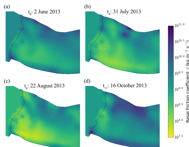
Figure 5. Basal friction coefficient obtained from inverse modelling and observed frontal position for (a) t_0 : 2 June 2013, (b) t_4 : 31 July 2013, (c) t_6 : 22 August 2013 and, (d) t_{11} : 16 October 2013.
