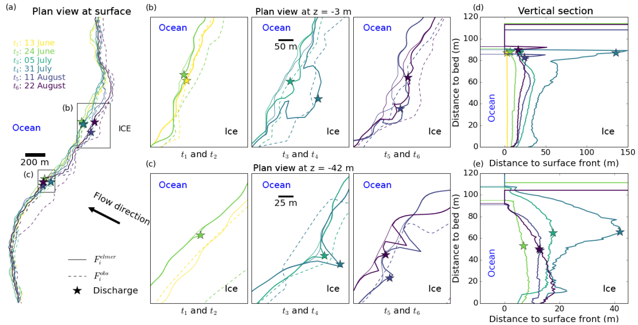
Figure 8. (a) Plan view of the observed frontal position of Kronebreen at six different dates, defined by different colours, corresponding to the satellite data acquisition dates during the melt season in 2013 (up to 22 August). At t_i , the observed front, F_i^{obs} , is represented by a dashed line and the advanced front, F_i^{elmer}(z=0) , by a thin line. The discharge location is defined by a star. Enlargement at (b) the northern discharge (ND) area at z = -3 m and at (c) the southern discharge (SD) area at z = -42 m with the advanced front at depth z where undercutting has been applied, F_i^{elmer}(z) , represented by a thick line. Vertical section (d) at the northern discharge (ND) location and at (e) the southern discharge (SD) location. The stars in (d, e) indicate the plan view elevation z from (b, c). Horizontal lines in (d, e) represent the sea level for each iteration.
