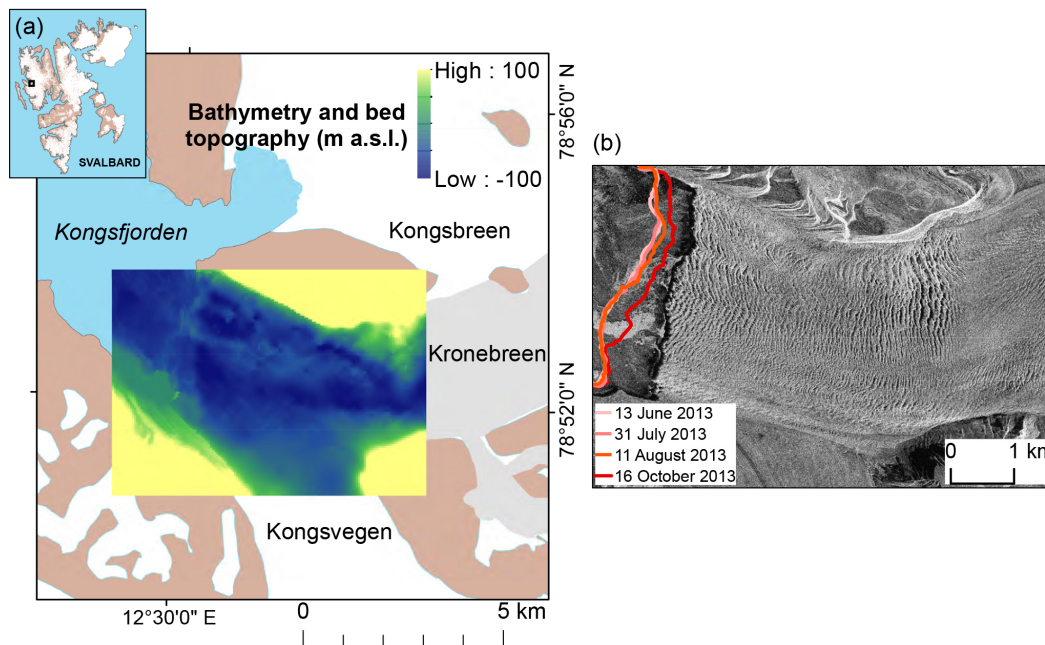
Figure 1. (a) Map of Kronebreen and its surrounding area. Ocean is in blue, bare rock is in brown and glacier ice is in white. The grey area represents the Kronebreen glacier system. The inset map in the top left shows the location of Kronebreen in Svalbard, and the central inset panel shows fjord bathymetry and bed topography in m.a.s.l. (b) Crevasse pattern at the front of Kronebreen in August 2014 from TerraSAR-X satellite (1 m resolution), and four frontal positions during 2013.
