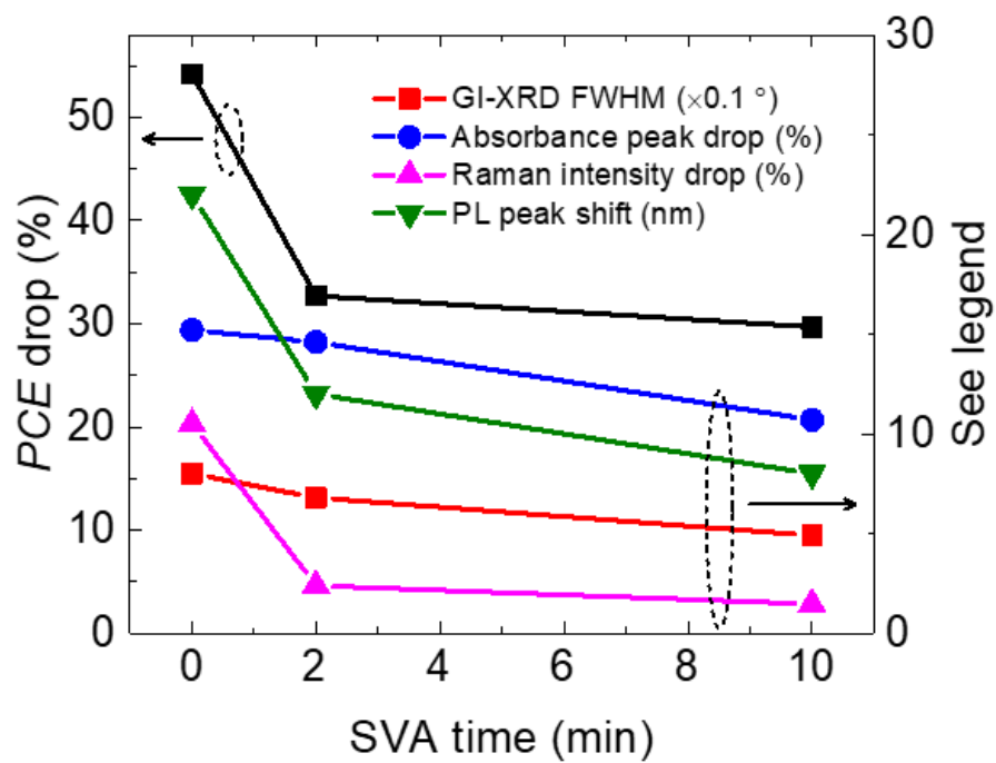
Figure 6 PCE drop, absorbance peak drop, relative Raman intensity drop, and PL peak shift after the photo-aging as a function of SVA time. For the GI-XRD FWHM, it is measured for fresh films (no obvious change after the photo-aging).
