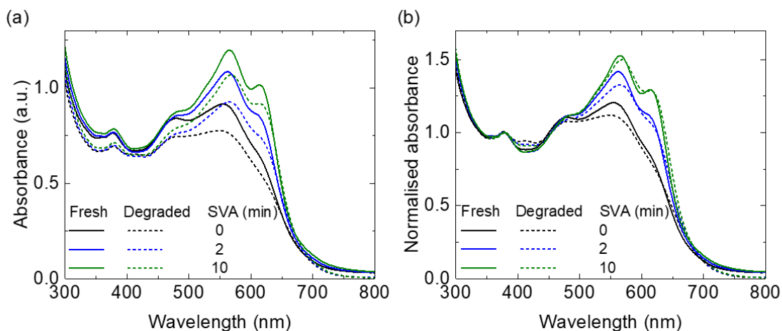
Figure 3. UV-Vis absorbance spectra of the fresh and photo-aged BTR:PC 71 BM films: 0 min SVA, 2 min SVA and 10 min SVA films (a) without normalisation, and (b) with normalisation to the PC 71 BM peak at 378 nm.
