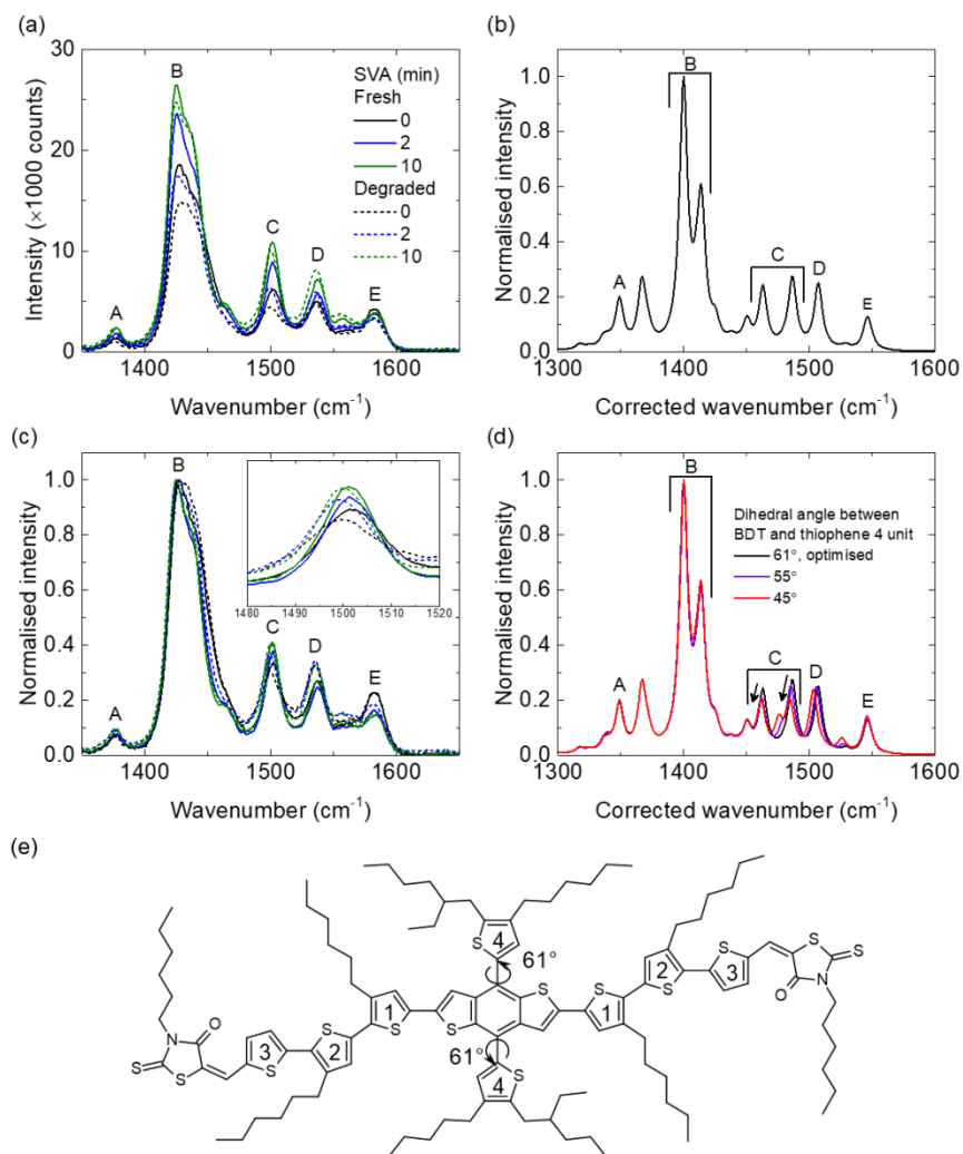
Figure 4 (a) Raman spectra of BTR:PC 71 BM films with increasing SVA time, before and after photo-aging, (b) calculated Raman spectrum of BTR using B3LYP 6311G(d,p) with all alkyl side chains simplified to methyl groups, (c) normalised Raman spectra of BTR:PC 71 BM films with increasing SVA time, before and after photo-aging (inset shows zoomed-in of peak C), (d) normalised calculated Raman spectrum of BTR with different dihedral angle between the BDT and thiophene 4 unit using the same simulation method, and (e) the chemical structure of BTR with numbered thiophenes for Raman peak assignment. The main backbone has dihedral angles ranging from \sim 15^\circ - 25^\circ . The thiophenes numbered as 4 are \sim 61^\circ out of the plane of the BDT core.
