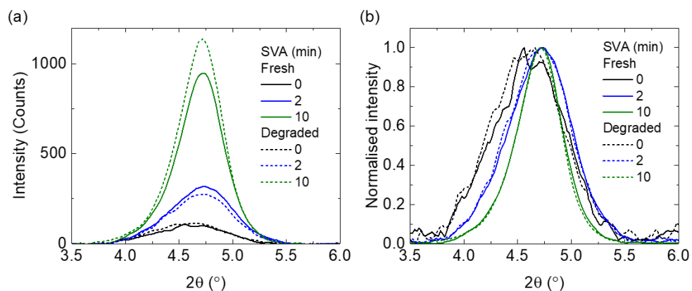
Figure 2. (a) GI-XRD spectra, and (b) normalised GI-XRD spectra, of BTR:PC 71 BM films with increasing SVA time, before and after photo-aging.
