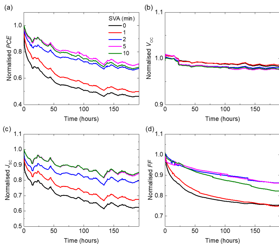
Figure 1. Normalised (a) PCE , (b) V_{OC} , (c) J_{SC} , and (d) FF (to the initial maximum values) of BTR:PC 71 BM devices, with active layers which have undergone increasing SVA time, as a function of photo-aging time under one sun equivalent illumination at room temperature in dry nitrogen.
