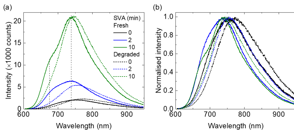
Figure 5 (a) PL spectra corrected by its absorbance at 532 nm (corresponding to the excitation wavelength), and (b) normalised PL spectra of BTR:PC 71 BM films with increasing SVA time before and after photo-aging.
