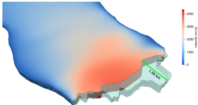
Figure 7. Rendering of model terminus showing large tabular calving event at 1.41 years of Run 111. Transparent region defines the geometry of the tabular berg (and additional concurrent bergs) released following the ice mélange collapse. The large tabular berg is 1.6 km long in the flow direction, with a mass of 1.14 Gt and a volume of 1.28 \times 10^9 \text{ m}^3 .
