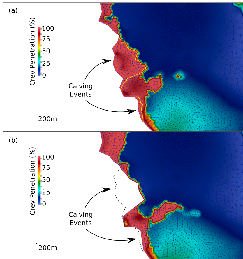
Figure 4. Crevasse penetration (%) on PlaneMesh. (a) Two concurrent calving events are delineated by yellow lines (the H_{crev} = 1 contour). (b) Crevasse penetration in subsequent time step. The calving events have expanded crevassing in the surrounding ice.
