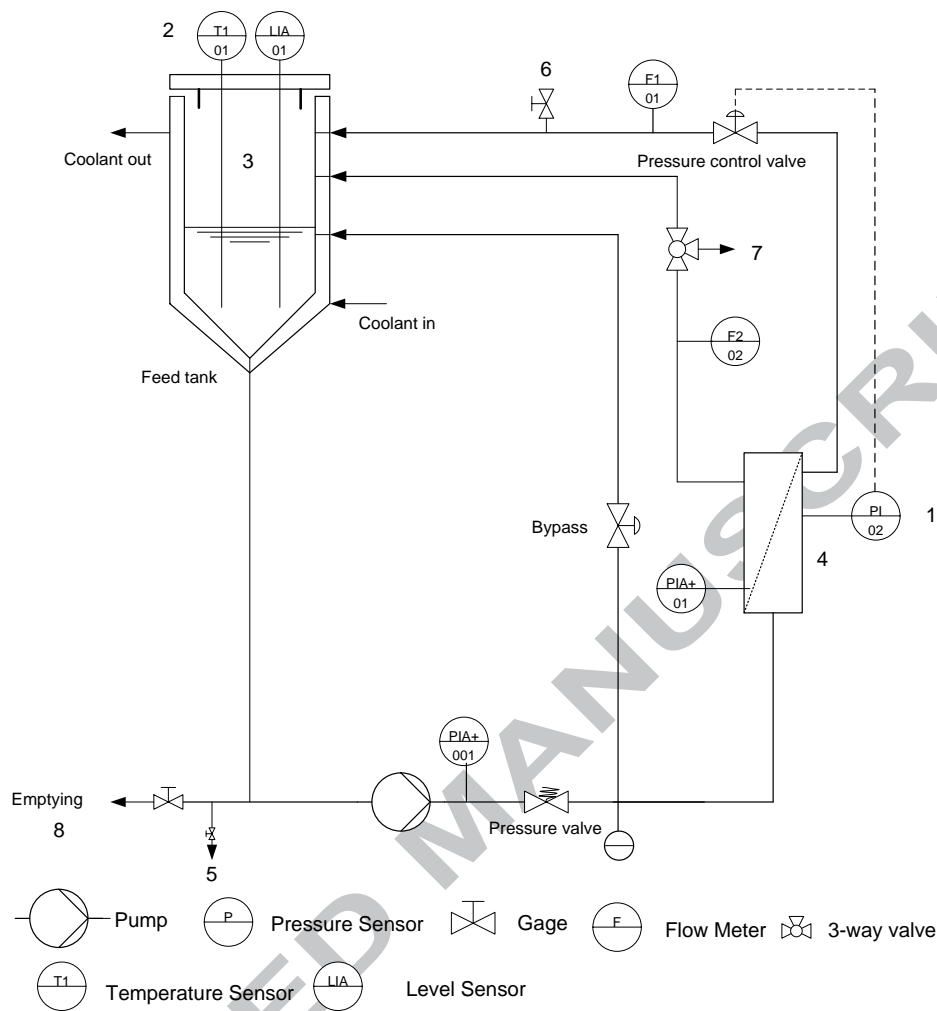
1: Pressure control, 2: Temperature control, 3: Feed tank, 4: Membrane module, 5: Permeate sampling valve, 6: Concentrate sampling valve, 7: Feed sampling valve, 8: drain valve
