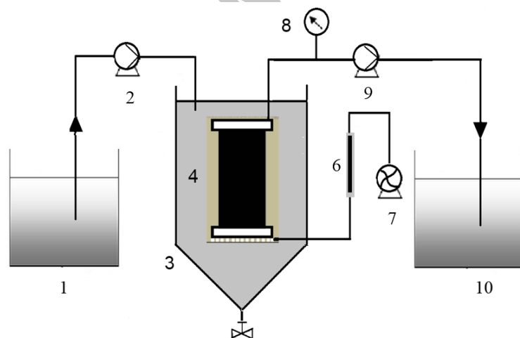
1: Feed tank; 2: Feed pump; 3: MBR reactor; 4: MBR module; 5: Exhaust valve; 6: Compressed air regulator; 7: Compressor; 8: Pressure sensor; 9: Suction pump; 10: Permeate collection tank
