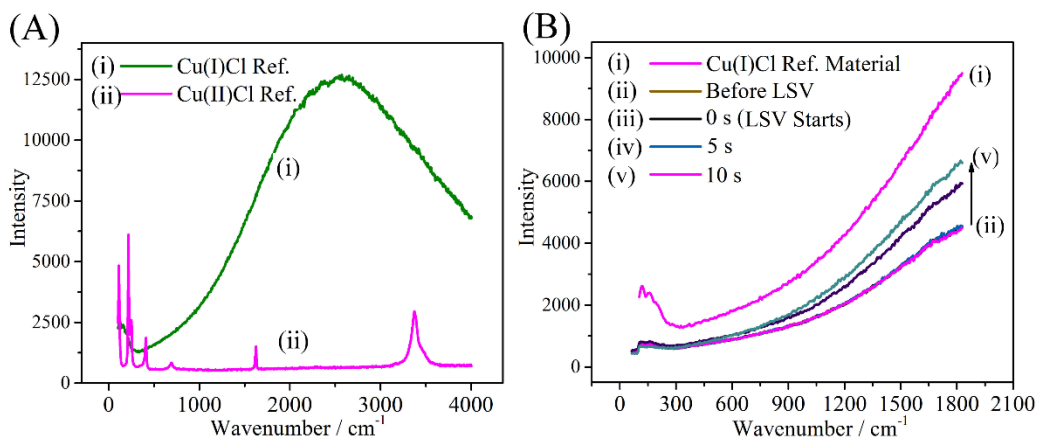
Figure 4. (A) Raman and fluorescence response for CuCl and CuCl 2 reference materials. (B) In situ Raman/fluorescence monitoring of the anodic corrosion reaction at a 125 \mu\text{m} diameter copper microelectrode immersed in 0.5 M NaCl(aq) with applied potential scanning (scan rate 20 \text{mV s}^{-1} ) from -0.2 V to +5.4 V vs. SCE to give Raman data sets for every 0.1 V interval (data shown only for data set at (iii) -0.2, (iv) -0.1, (v) and 0.0 V vs. SCE).
