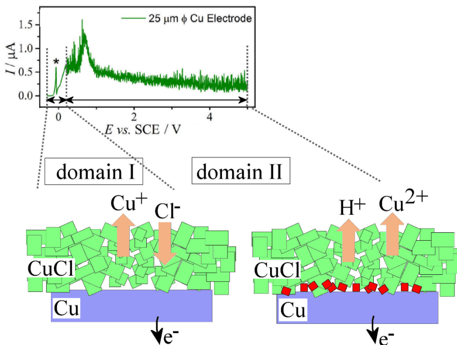
Figure 11. Schematic drawing of the surface redox processes associated with domain I (at lower applied potential) and domain II (at higher applied potential) and the corresponding ion transport processes in the CuCl blocking layer.
