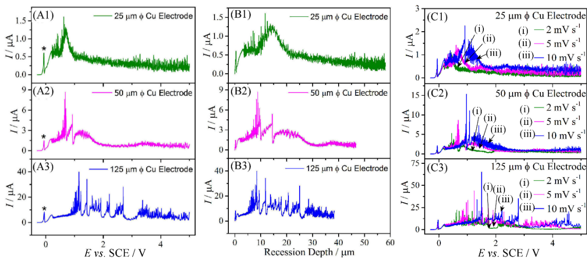
Figure 6. (A) Linear sweep voltammograms (scan rate 5 \text{mV s}^{-1} ) from -0.3 to +5.0 V vs. SCE at (A1) 25, (A2) 50, and (A3) 125 \mu\text{m} diameter copper microelectrodes immersed in 0.5 M NaCl (the initial Cu(I/0) anodic peak is labelled with an asterisk). (B) As above, but data replotted versus recession depth, which has been estimated based on a copper density of 8.93 \text{g cm}^{-3} . (C) As above but for a scan rate of 2, 5, and 10 \text{mV s}^{-1} .
