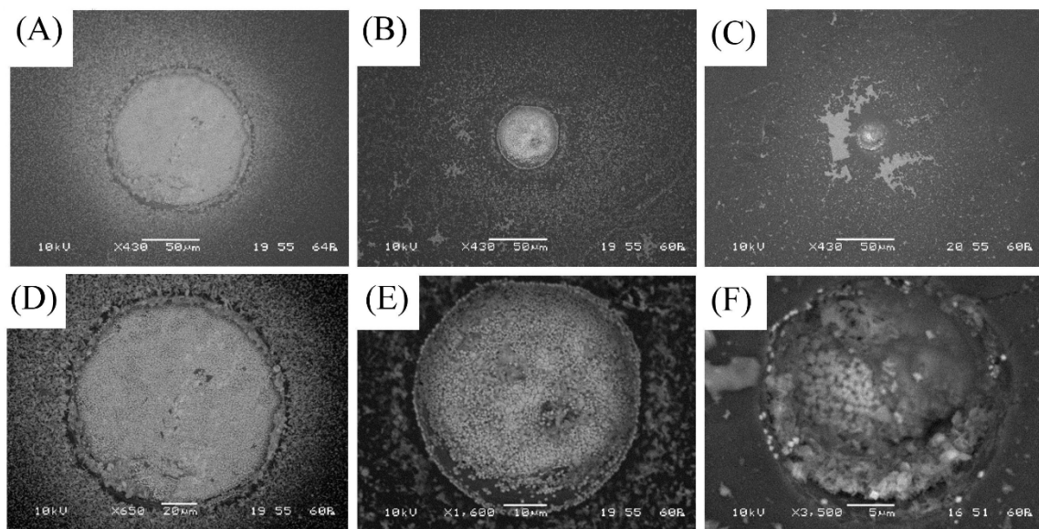
Figure 7. Scanning electron microscopy (SEM) images for copper microelectrodes of diameters (A,D) 125 \mu\text{m} , (B,E) 50 \mu\text{m} , and (C,F) 25 \mu\text{m} after linear sweep voltammetry from -0.3 V to 5.0 V vs. SCE at 5 \text{mV s}^{-1} . Images A-C are scaled to images D-F to reveal more details.
