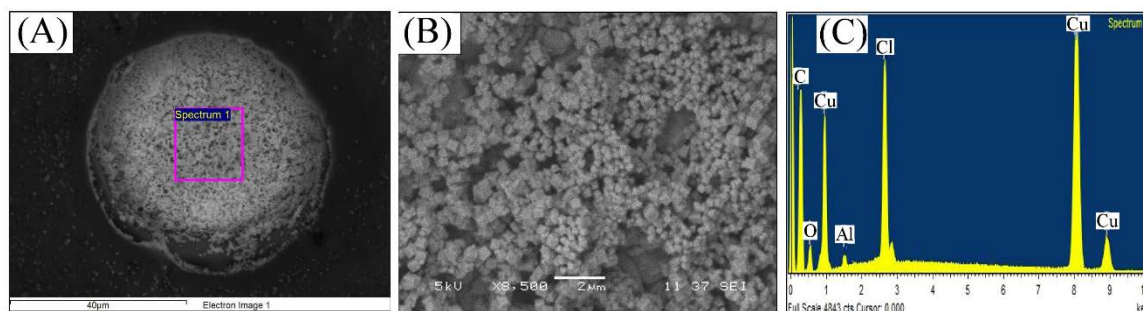
Figure 8. (A,B) SEM images of the surface of a 50 \mu\text{m} diameter Cu microelectrode after linear sweep voltammetry from -0.3\text{ V} to 5.0\text{ V} vs. SCE at 5\text{ mV s}^{-1} in 0.5\text{ M NaCl} . (C) Energy-dispersive X-ray elemental analysis (EDX) for the area indicated in (A).
