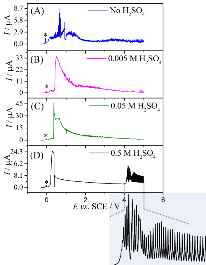
Figure 9. (A) Linear sweep voltammograms (scan rate 5 \text{ mV s}^{-1} ) from -0.3 to +5.0 \text{ V vs. SCE} at a 50 \text{ }\mu\text{m} diameter copper microelectrode immersed in 0.5 \text{ M NaCl} (the initial \text{Cu(I/O)} anodic peak is labelled with an asterisk). (B) As above with 5 \text{ mM H}_2\text{SO}_4 added. (C) As above with 50 \text{ mM H}_2\text{SO}_4 added. (D) As above with 500 \text{ mM H}_2\text{SO}_4 added. Inset showing onset of oscillations.
