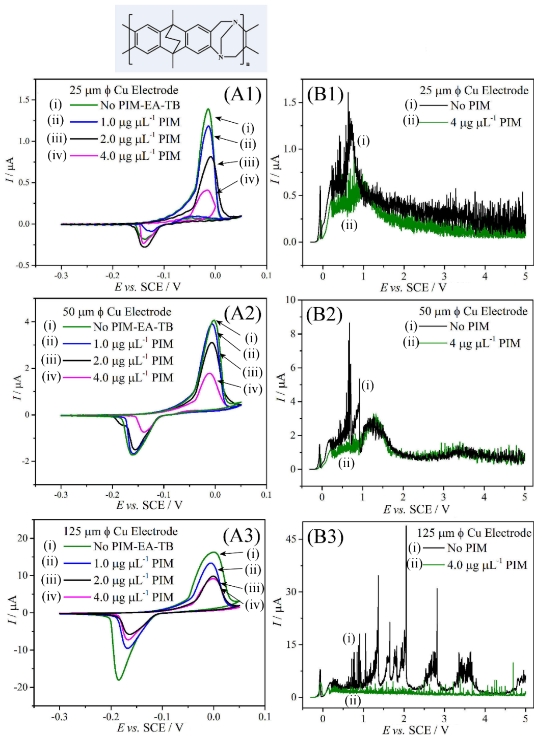
Figure 10. (A) Cyclic voltammograms (scan rate 100 \text{ mVs}^{-1} ) for a (A1) 25, (A2) 50, and (A3) 125 \mu\text{m} diameter copper microelectrode with different amounts of PIM-EA-TB deposited and immersed in 0.5 \text{ M NaCl} . Inset showing the molecular structure of PIM-EA-TB. (B) Linear sweep voltammograms (scan rate 5 \text{ mVs}^{-1} ) for a (B1) 25, (B2) 50, and (B3) 125 \mu\text{m} diameter copper microelectrode without/with 4.0 \mu\text{g } \mu\text{L}^{-1} PIM-EA-TB coating immersed in 0.5 \text{ M NaCl(aq)} .
