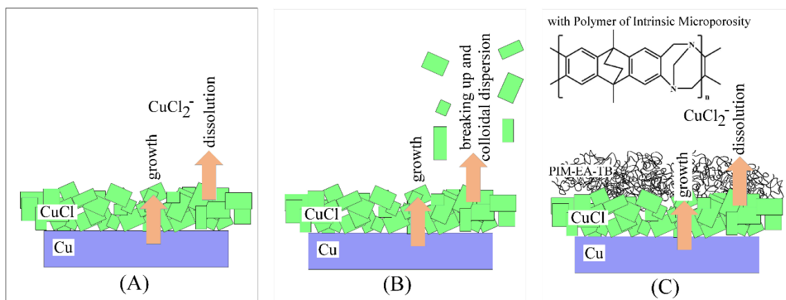
Figure 1. Graphical illustration of (A) the CuCl precipitation-dissolution mechanism suggested to be responsible for oscillatory behavior in acidified chloride media, (B) the redox driven Cu(II)/Cu(I) destabilization of CuCl observed in neutral chloride media associated with colloidal break-up of the CuCl film, and (C) the process when investigated under a coating of PIM-EA-TB to prevent colloidal break-up.
