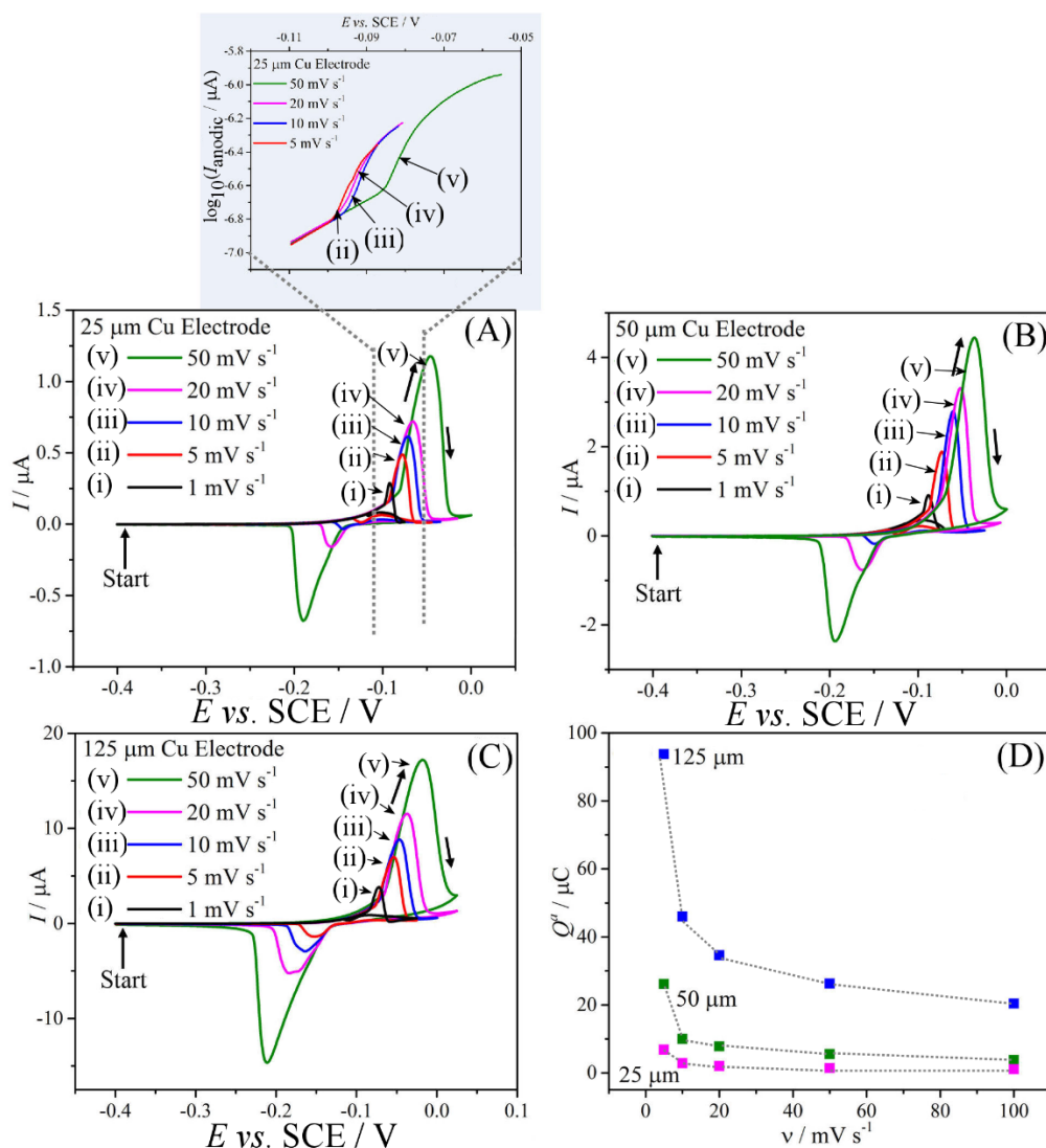
Figure 3. Cyclic voltammograms at 1, 5, 10, 20 and 50 \text{mV s}^{-1} scan rates in 0.5 M NaCl(aq) for (A) 25 \mu\text{m} , (B) 50 \mu\text{m} , and (C) 125 \mu\text{m} diameter (epoxy-mounted) copper electrodes. (D) Plot of anodic charge, Q^{\text{ox}} versus scan rate ( v ) is given for each electrode size.
