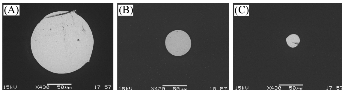
Figure 2. SEM images of polished copper microelectrodes of diameters (A) 125 \mu\text{m} , (B) 50 \mu\text{m} , and (C) 25 \mu\text{m} before use.
