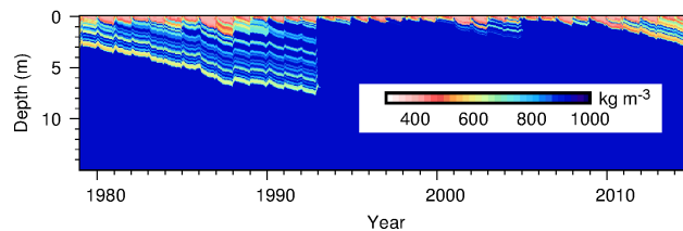
Figure 6. Time evolution of firm density as a function of depth for Cabinet Inlet, predicted by the firm density model (Ligtenberg et al., 2011).
