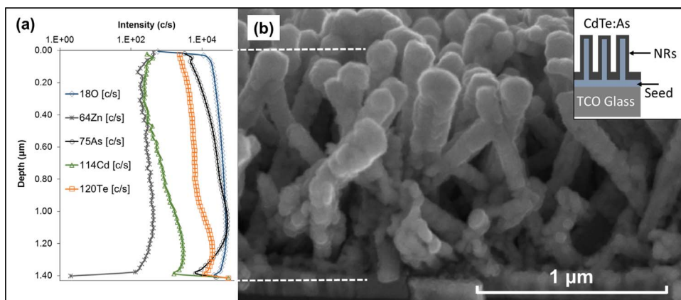
Fig. 5. SIMS depth profiles of the Zn^{64} , O^{18} , Cd^{114} , Te^{120} , and As^{75} isotopes (a) and a cross-sectional SEM image (b) for a CdTe:As coated ZnO NR array with rod length of \sim 1.4 \mu\text{m} .
