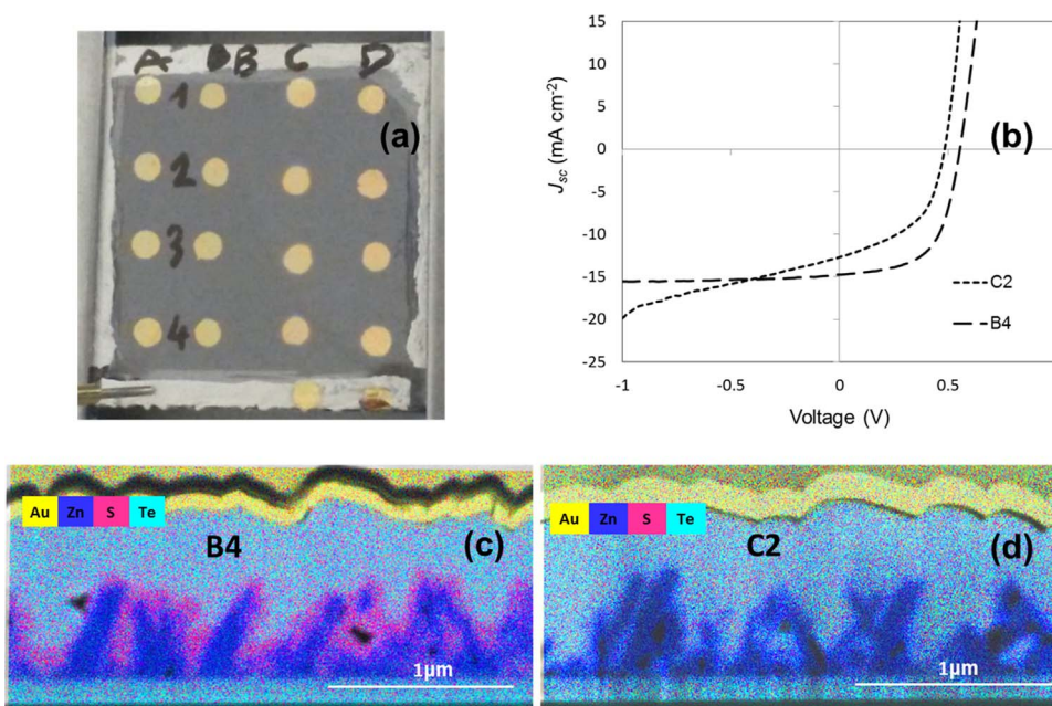
Fig. 7. A typical 2.5 \times 2.5 \text{ cm}^2 CdTe/CdS/ZnO NRs device with 2 mm diameter dot contacts (a), light J - V curves (b) and cross-sectional EDS elemental (Au, Zn, S, and Te) maps (c, d) for selected cells (B4, C2). ZnO NRs in cell B4 have a CdS coating whereas those in C2 has little/or no CdS coverage. The ZnO NRs are embedded in a relatively thick CdTe layer electrically separating the Au contact.
