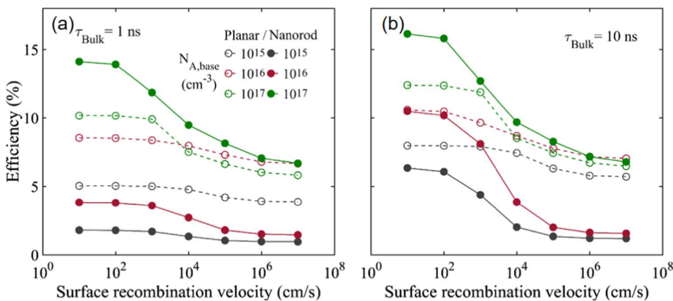
Fig. 9. Calculated efficiencies of planar and NR-based CdTe solar cells with bulk doping concentrations of 1 \times 10^{15} , 1 \times 10^{16} and 1 \times 10^{17} \text{cm}^{-3} and bulk lifetimes of (a) 1 ns and (b) 10 ns with respect to CdTe/CdS surface recombination velocity. Solid and dashed lines are provided to guide the eye.
