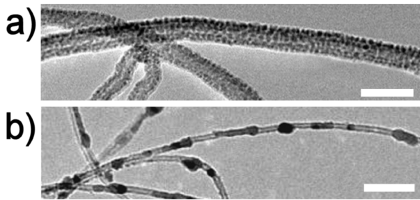
FIG. 1: TEM micrographs of multiwall CNTs with a nickel coating. a) Nominal 5 nm nickel layer sputtered at 20°C, showing small clusters with a high nucleation density. The scale bar corresponds to 40 nm. b) Nickel layer upon heating to 660°C for 2 min. Larger clusters coexist with segments of continuous coating on the nanotube. The scale bar corresponds to 100 nm.
