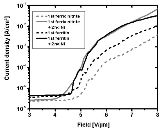
FIG. 5: Field emission measurements on nanotube samples. Comparison of the field emission obtained for samples with ferritin catalyzed primary CNTs (black lines), with and without nickel catalyzed secondary CNTs. Idem for samples with ferric nitrate catalyzed primary CNTs (gray lines), with and without nickel catalyzed secondary CNTs.
