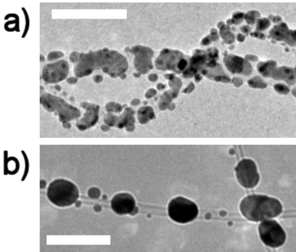
FIG. 3: TEM micrographs of multiwall CNTs with a gold coating. a) Nominal 5 nm gold layer sputtered at 20°C, showing gold islands with an arbitrary shape. b) Same Au layer after heating to 660°C for 2 min, showing the formation of sphere-like clusters which have a small contact area with the nanotubes. Scale bars correspond to 50 nm.
