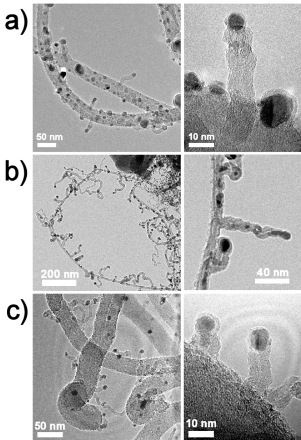
FIG. 4: TEM micrographs of secondary CNTs grown on the sidewalls of primary CNTs. a) Secondary nickel catalyzed CNTs grown on relatively thick primary ferric nitrate catalyzed CNTs. b) Secondary nickel catalyzed CNTs grown on thin primary ferritin catalyzed CNTs. c) Secondary ferritin catalyzed CNTs grown on primary ferric nitrate catalyzed CNTs.
