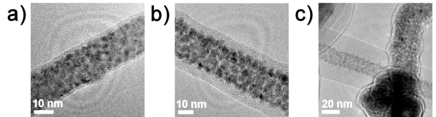
FIG. 2: TEM micrographs of ferric nitrate catalyzed CNTs with nominal a) 5 nm, b) 10 nm and c) 15 nm nickel coating. A cluster-like nickel under-layer is visible, with a more electron transparent continuous nickel top-layer. The electron transparency is especially in c) clearly observable.
