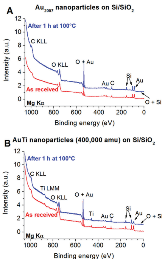
Fig. 1 XPS spectra of Au 2057 (A) and Au/Ti (B) nanoclusters deposited on Si/SiO 2 slabs before and after 100 °C for 1 h in 1 bar of O 2 :CO = 4:1 mixture. Spectra were calibrated for Au 4f 7/2 line to appear at binding energy of 84 eV and were normalized with the area of the Si 2s peak. The plots were offset in y direction for better visibility.
