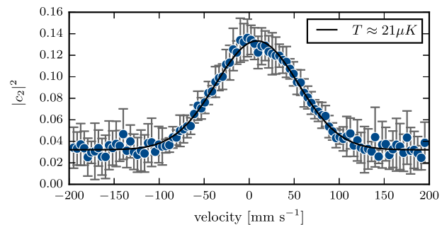
Figure 4. Velocity distribution measured by low intensity Raman velocimetry. A thermal distribution with a temperature of 21\ \mu\text{K} sits atop a broad background attributed to inhomogeneous sub-Doppler cooling (4, 24).
