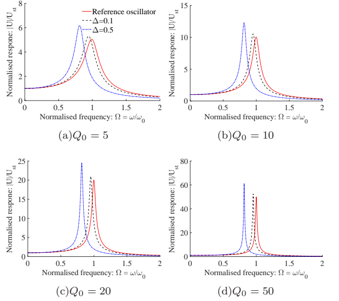
Fig. 6. Normalised response amplitude of the oscillator in the frequency domain as a function of the normalised frequency \Omega = \omega/\omega_0 for two different mass absorption factors \Delta and four different Q-factors.
