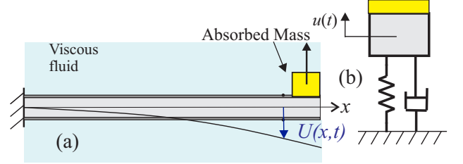
Fig. 1. Schematic diagrams of: (a) A cantilever micromechanical mass sensor immersed in a viscous fluid, and (b) An equivalent damped single degree of freedom model oscillator model.
