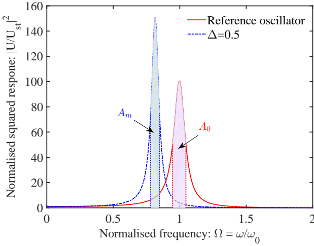
Fig. 9. Squared-response of the reference oscillator and the mass-absorbed oscillator for \Delta = 0.5 and Q_0 = 10 . The shared areas A_m and A_0 represent the area within the half-power bandwidths, expressed as
