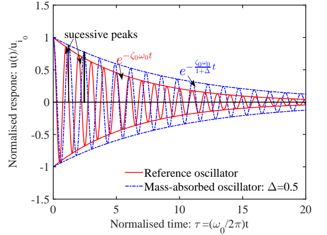
Fig. 5. Normalised response of the oscillator in the time domain due to an initial displacement plotted as a function of normalised time \tau = t/T_0 for mass absorption factor \Delta = 0.5 and Q_0 = 20 .
