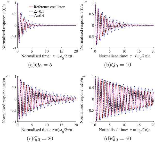
Fig. 4. Normalised response of the oscillator in the time domain due to an initial displacement plotted as a function of normalised time \tau = t/T_0 for two different mass absorption factors \Delta and four different Q-factors.
