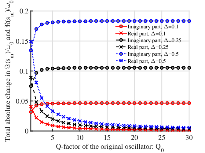
Fig. 3. The absolute change in the real and imaginary parts of the complex frequency (normalised by \omega_0 ) due to the addition of mass as a function of the Q-factor of the reference oscillator.
