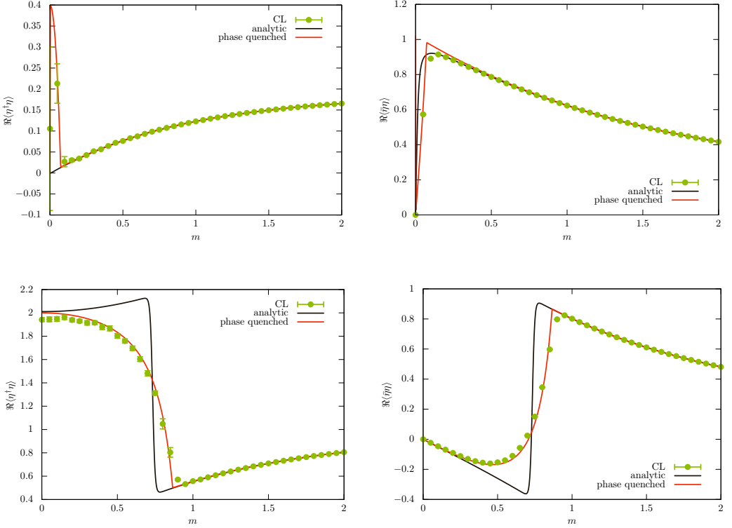
Figure 4. Mass scan for \mu = 0.2 (upper panel) and \mu = 1 (lower panel) for matrices with N = 48 . In both cases we plot the baryon number density on the left and the chiral condensate on the right.
