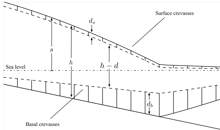
Figure 1. Sketch of the vertically integrated continuum damage model. The full thickness of the ice sheet ( h ) is divided into three layers. The upper and lower layers are assumed to be entirely riven by surface crevasses of depth d_s and basal crevasses of depth d_b , while the layer between them (with thickness h - d = h - (d_s + d_b) ) is considered intact. The crevassed layers offer no resistance to horizontal longitudinal and lateral shearing but behave in the same way as undamaged ice with regard to isotropic compression and vertical shear.
