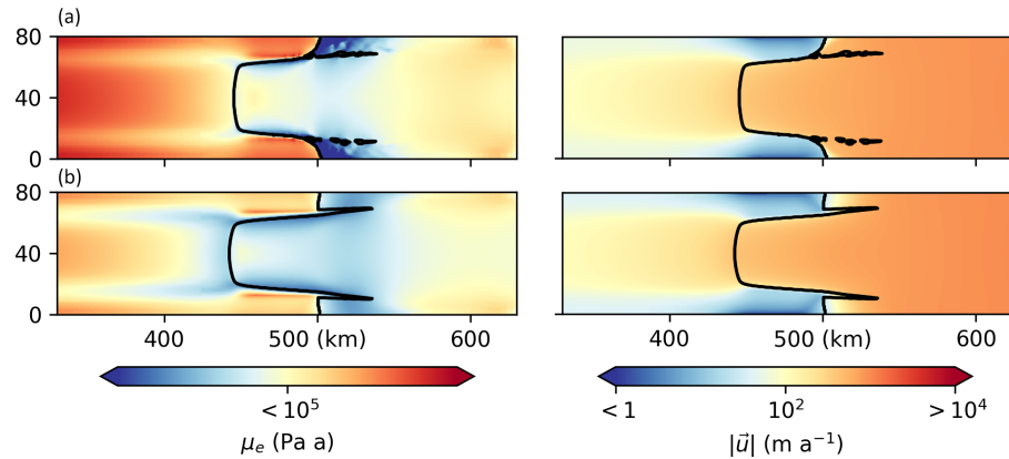
Figure 4. Comparison of the final IceD0 (a) and Ice0 (b) patterns of vertically averaged effective viscosity ( \mu_e ) and speed ( |\bar{u}| ). The impact of damage on effective viscosity varies both laterally and between grounded and floating ice, but the shape and position of the grounding line (solid black contour) of IceD0 are similar to those of Ice0, as is the velocity field. These are approximately steady-state patterns as the grounded area and volumes change very little after 1000 years (see also Figs. 7 and 8).
