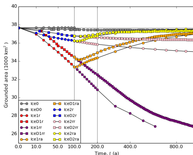
Figure 7. Grounded area against time for all of the simulations. Lines with circles show the results based on BISICLES without the damage model and those with squares show the results based on BISICLES with the damage model. Grey curves show the results of the control run Ice0, IceD0; red curves show the results of Ice1r, IceD1r; orange curves show the results of Ice1ra, IceD1ra; purple curves show the results of Ice1rr, IceD1rr; blue curves show the results of Ice2r, IceD2r; yellow curves show the results of Ice2ra, IceD2ra; pink curves show the results of Ice2rr, IceD2rr. BISICLES_D produces slightly less retreat than BISICLES.
