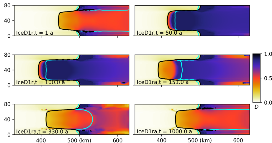
Figure 5. Comparison of the retreat and recovery due to changes in ice shelf basal melt (IceD1rr and IceD1ra) in MISIP+. IceD1r sees the grounding line (solid black contour) in the centre of the channel retreat to x = 390 km over 100 years in response to strong ablation across the whole ice shelf. Parts of the ice shelf are thin ( h < 200 m, outside cyan contour) so that a high value of \bar{D} implies only a small reduction in buttressing from those regions. IceD1ra follows directly from IceD1r, setting the melt rate to zero so that the ice shelf thickness and the grounding line readvances, recovering its original shape after around 1000 years.
