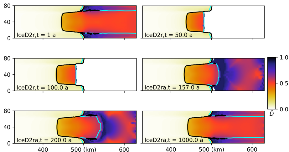
Figure 6. Comparison of the retreat and recovery due to changes in calving front position (experiments IceD2rr and IceD2ra in MISIMIP+). A melt rate of 100 \text{ m a}^{-1} is applied, where x > 480 \text{ km} results in a remnant ice shelf whose damage field resembles the initial state in their common area but grows somewhat toward the front (IceD2r). Loss of buttressing leads to grounding line (solid black contour) retreat. Once the melt rate is set to zero (IceD2ra) the calving front advances, carrying a region of elevated damage with it across the domain edge. Thin, damaged ice downstream from the h = 200 \text{ m} contour (cyan) forms from direct accumulation on the sea surface.
