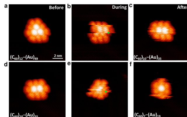
Figure 2. Tip-triggered cascade cluster transformation. (a–c) Transformation from (C_{60})_{12}-Au_{49} to (C_{60})_{10}-Au_{35} . (d–f) Transformation from (C_{60})_{10}-Au_{35} to (C_{60})_7-Au_{19} . Green dots in (b) and (e) indicate the locations where the tip is driven toward the C_{60} molecule.
