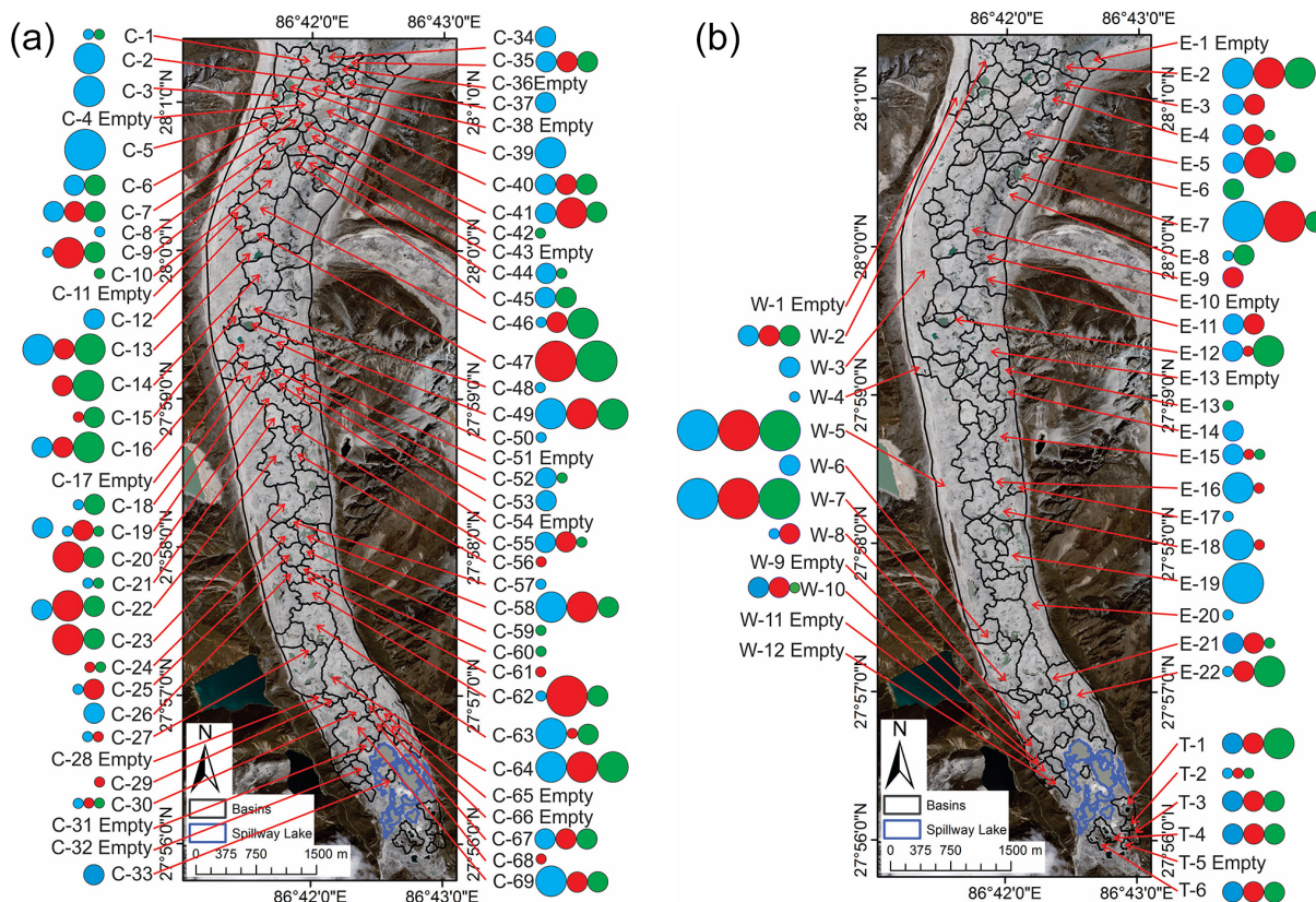
Figure 10. Surface drainage basins and lake area changes: (a) the central part of the glacier and (b) the lateral margins and terminal zone. Lake areas are shown for 2010 (blue), 2012 (red), and 2015 (green) in four categories: < 1000 \text{ m}^2 (small circles), 1000\text{--}5000 \text{ m}^2 (medium circles), 5000\text{--}10\,000 \text{ m}^2 (large circles), and > 10\,000 \text{ m}^2 (largest circles). Missing coloured circles indicate empty basins in that year.
