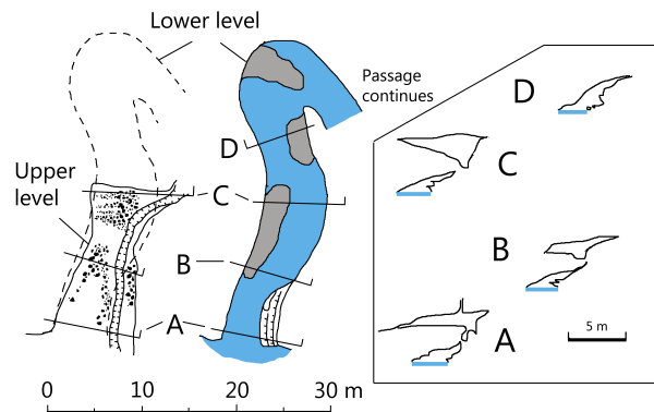
Figure 6. Plan and passage cross sections of conduit NG-05. The plan view of the upper level shows boulders and an incised channel on the conduit floor. For location see Fig. 3a.
