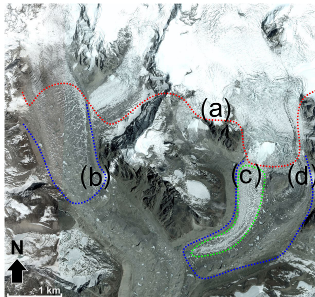
Figure 9. Distribution of crevasses on the W and NE branches of Ngozumpa Glacier. (a) Lower boundary of crevasse fields; (b, c, d) areas where supraglacial channels occur on debris-covered and clean (c) ice. Image source: Google Earth.
