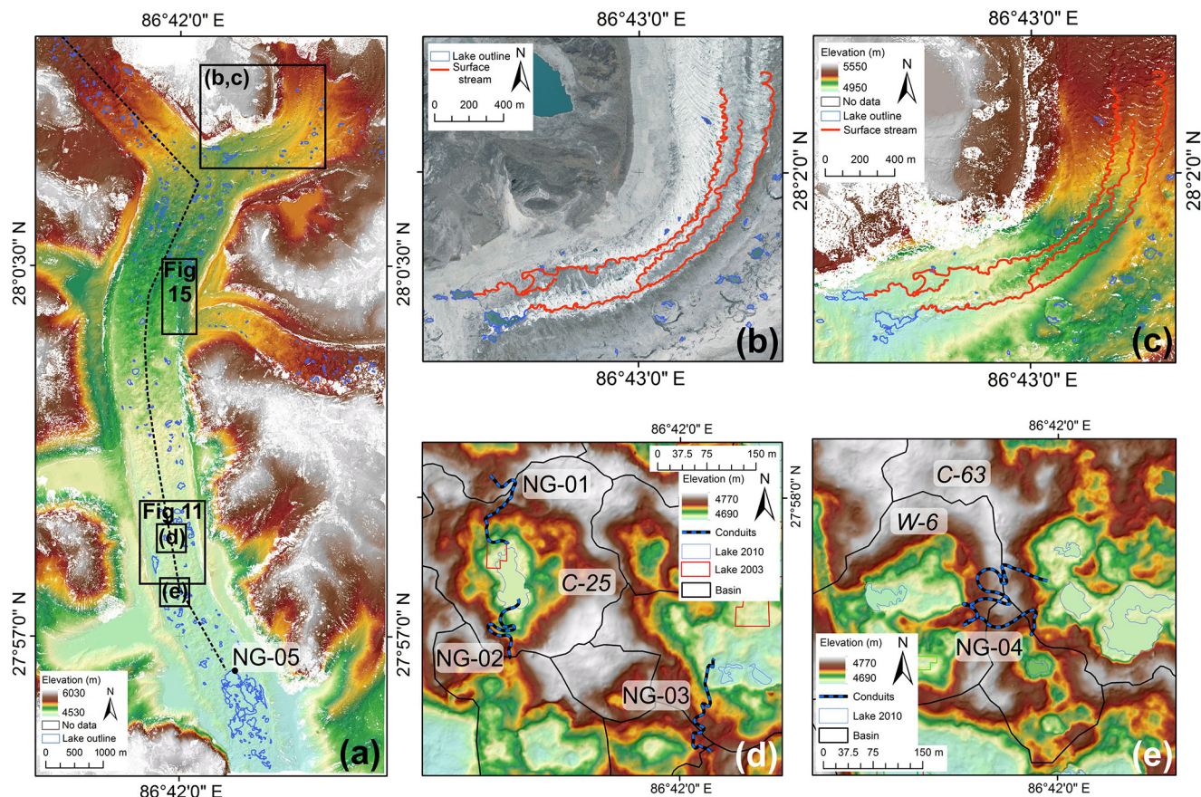
Figure 3. Examples of surface topography, supraglacial meltwater channels, and englacial conduit locations on Ngozumpa Glacier: (a) DEM of the lower ablation zone of the glacier, based on GeoEye-1 stereo imagery from June 2010, showing location of enlarged panels and englacial conduit NG-05; (b) supraglacial channels shown on the 2010 imagery; (c) the same area shown on the 2010 DEM; (d) hummocky debris-covered ice, showing the boundaries of closed surface basins and locations of englacial conduits NG-01 to NG-03 (considerable basin expansion occurred in the four ablation seasons between the conduit surveys (December 2005) and the date of the DEM (June 2010)); and (e) hummocky debris-covered ice and location of englacial conduit NG-04 (surveyed November 2009, 7 months before the date of the DEM). The dashed line in panel (a) shows the location of the long profile in Fig. 2.
