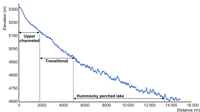
Figure 2. Longitudinal surface profile of the W branch and main trunk of Ngozumpa Glacier, showing downglacier changes in gradient and relative relief (see Fig. 3a for location). “Upper channeled”, “transitional”, and “hummocky perched lake” refer to the drainage zones described in Sects. 4.2 and 4.3.
