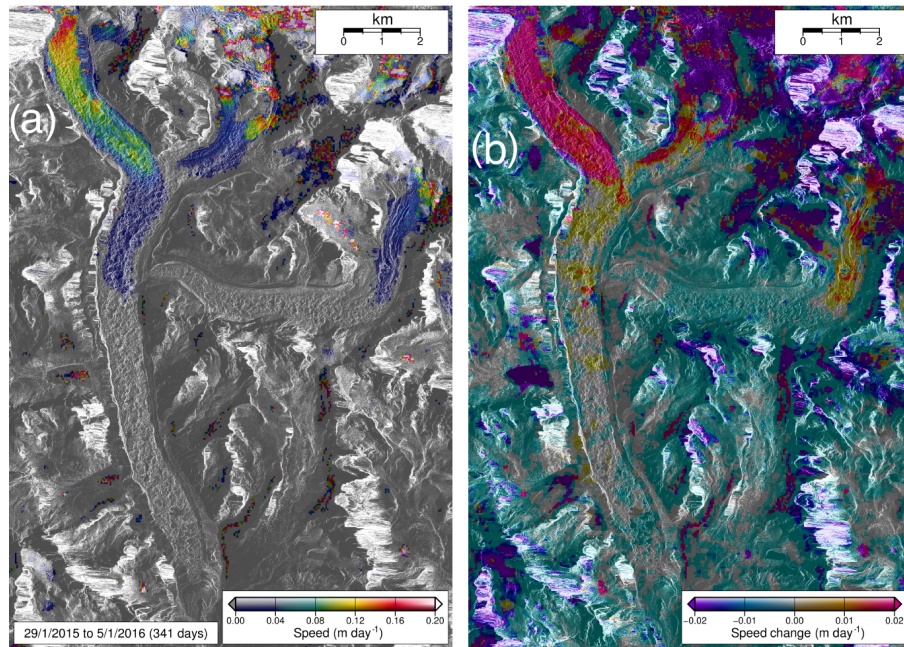
Figure 8. Surface velocities derived from TerraSAR-X data: (a) mean daily velocity for the “annual” period (29 January 2015 to 5 January 2016); (b) velocity difference between “annual” period (29 January 2015 to 5 January 2016) and “winter” period (19 September 2014 to 18 January 2015), indicating minimum summer speed-up of the glacier. No masks or filters were applied to the data.
