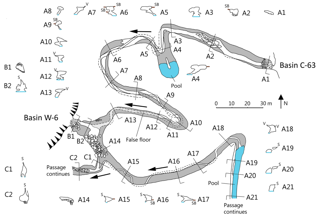
Figure 4. Plan and passage cross sections of englacial conduit NG-04. SB: sediment band; S: suture; V: voids. Dark-grey-filled and white-filled areas within the cave plan indicate the floors of the upper and lower levels, respectively. Pale grey and dashed lines are used where the lower level is occluded by higher false floors. Standing water on the cave floor is shown in blue. For location, see Fig. 3e.
