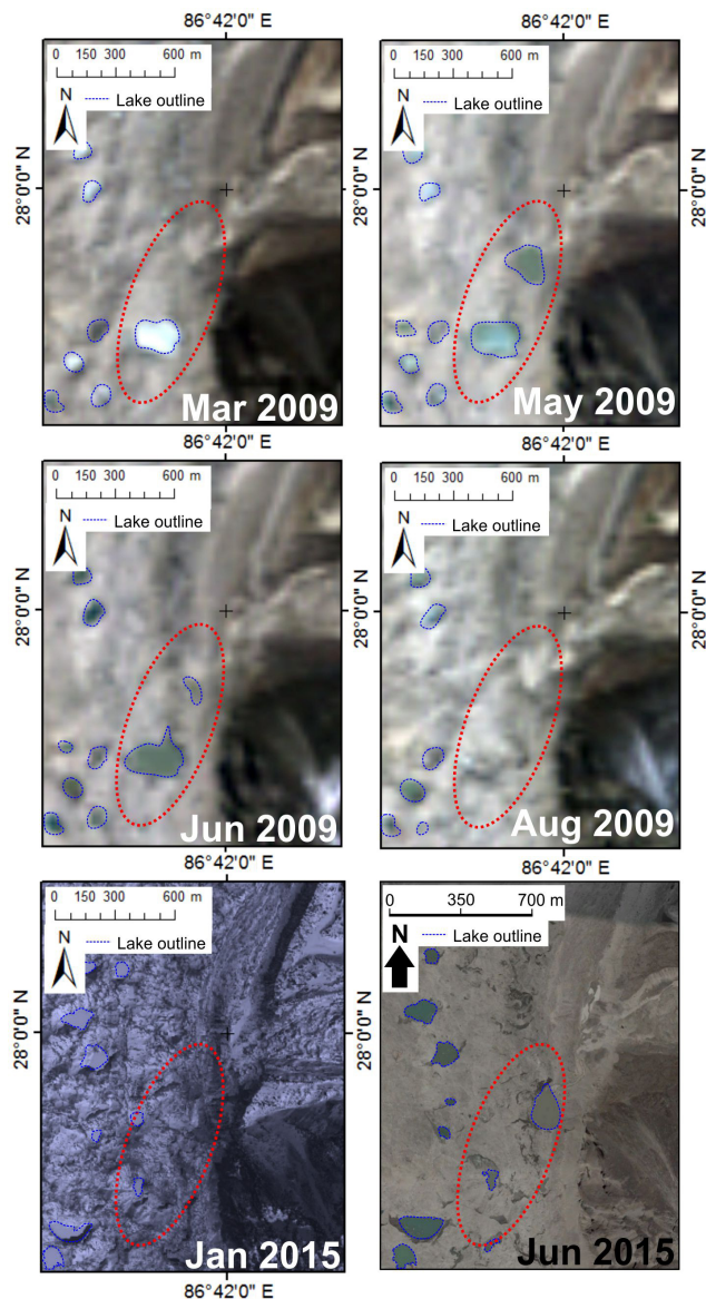
Figure 12. Changing pond extent in basin E-11, showing evidence of filling and drainage cycles. Pond outlines highlighted in blue.
