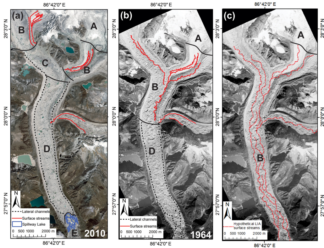
Figure 14. Zonation of the drainage system in (a) 2010 and (b) 1964, and (c) a hypothetical configuration at the Little Ice Age maximum. A: crevasse fields; B: supraglacial channels; C: transitional zone with shallow basins; D: closed surface basins with perched lakes; E: Spillway Lake. Dashed black lines indicate the positions of sub-marginal conduits.
