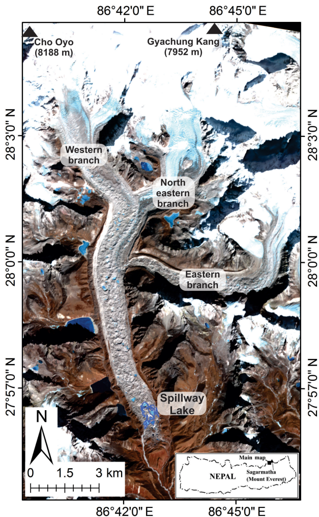
Figure 1. Ngozumpa Glacier, showing the location of the three branches and Spillway Lake. Image: orthorectified GeoEye-1 from December 2012.
