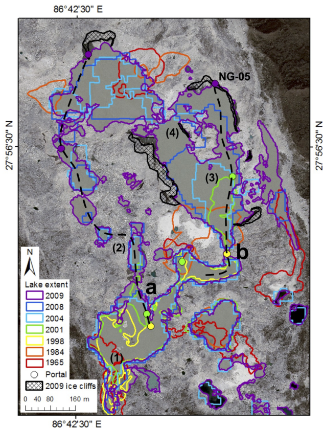
Figure 13. Spillway Lake, 1965–2009, showing the position of meltwater portals and upwellings and the inferred location of former englacial conduits (dashed lines). Background image: GeoEye-1 from June 2010. See text for explanation of lake evolution.
