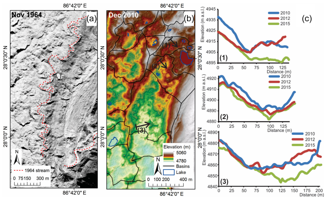
Figure 15. Evolution of the eastern margin of the main trunk of Ngozumpa Glacier, 1964–2015. (a) Supraglacial streams on the glacier surface in 1964 Corona imagery; (b) 2010 DEM, showing surface basins and the location of profiles; (c) surface profiles in 2010, 2012, and 2015, showing patterns of downwasting.
