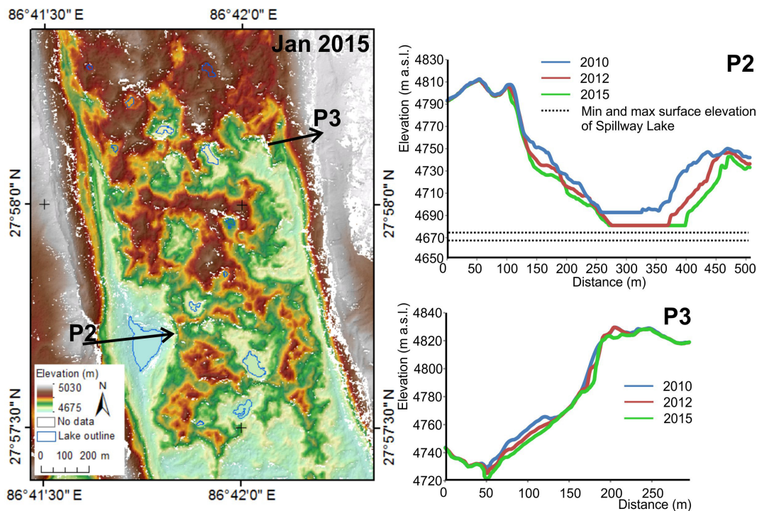
Figure 11. Extract from the 2015 DEM and selected cross profiles in 2010, 2012, and 2015, showing lateral troughs, subsidence of trough floors, and erosion of moraine slopes.
