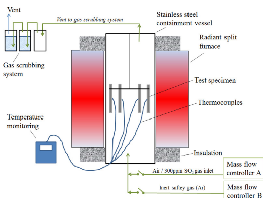
Fig. 4. Schematic illustration of the hot corrosion chamber used to corrode salt coated test specimens in an air-300 ppm \text{SO}_2 environment at 700 °C.
