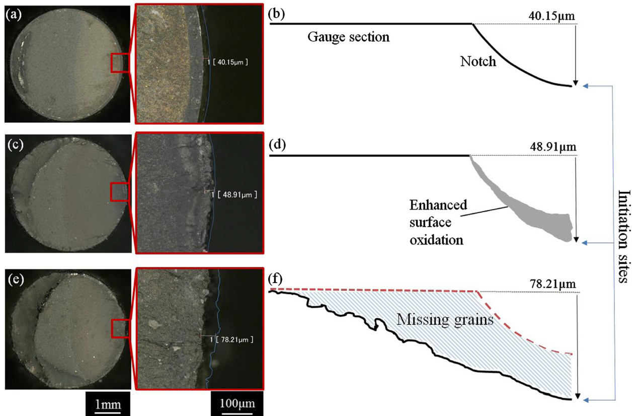
Fig. 9. Fracture surface and corresponding cross sectional schematic respectively of (a), (b) pre-notched specimen fatigue tested at high stress (c), (d) pre-notched and corroded fatigue specimen tested at low stress and (e), (f) pre-notched and corroded fatigue specimen tested at high stress.
