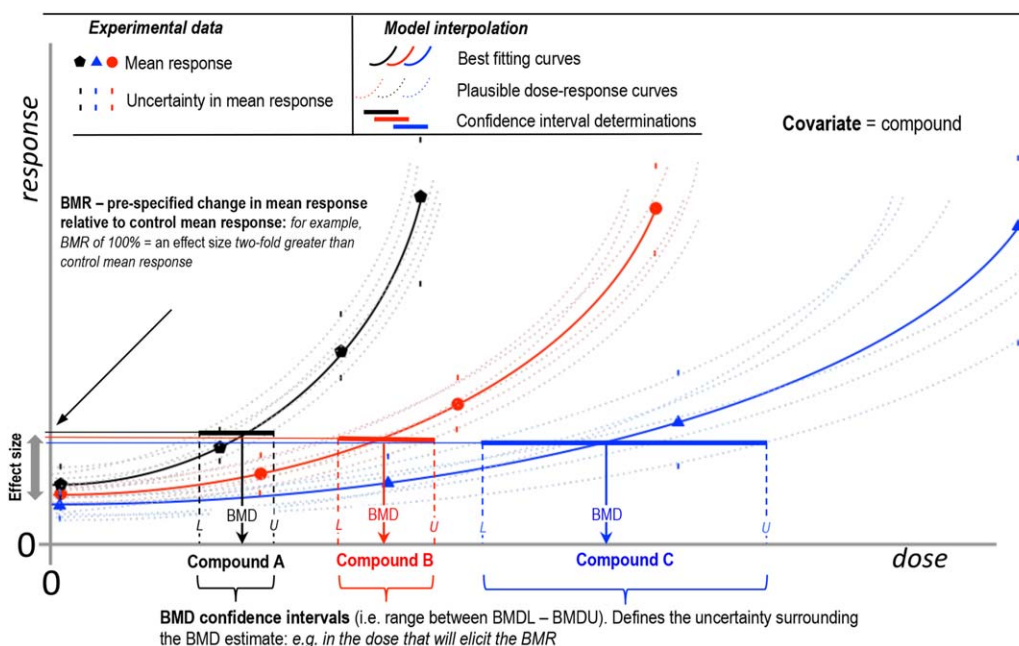
Fig. 1. Schematic overview of the BMD combined covariate approach. The benchmark dose approach (BMD) provides an estimate of the dose that will elicit a small, pre-specified effect-size called the benchmark response (BMR). The best-fitting BMD model (solid curve) will result in the best estimate of the BMD. Importantly however, the uncertainty in the dose-response data needs to be accounted for through calculation of a BMD confidence interval. The process can be conceptually visualized by imagining that, through variation of the model parameters, other curves, and BMDs that plausibly describe the data (e.g., schematically represented by the dashed curves) may be established. Together these values comprise the BMD confidence interval (solid line). In turn, this process provides estimations of the BMDL (L) and BMDU (U), the lower and upper 90% confidence bounds of the BMD estimate, respectively.
