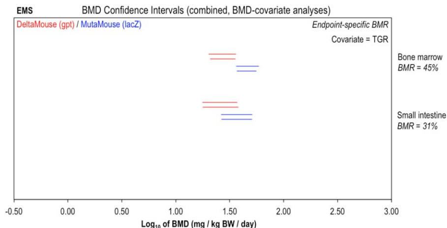
Fig. 3. Genotoxic potency of ethyl methanesulphonate (EMS) determined using the gpt delta mouse (red) and Muta TM Mouse (blue) transgenic rodent assays: endpoint-specific BMRs. BMD analysis, with endpoint-specific BMR values, was conducted to compare BMDs determined across two TGR assay variants. Two-sided 90% confidence intervals of the BMD, based on BMRs indicated beneath each tissue, were calculated from mutant frequency (MF) dose-response data (i.e., gpt or
