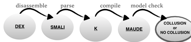
Fig. 8: Work-flow for the Android formal semantics in the \mathbb{K} framework.
