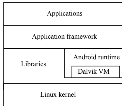
Fig. 1: Android operating system layers
