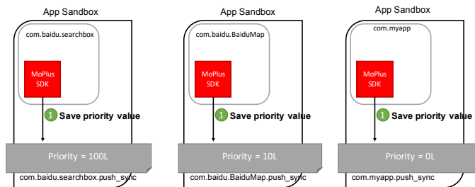
Fig. 3: Phase 1 of the colluding behaviour execution. Each app saves a priority value that depends on the amount of access it has to the system resources. Priority values are shown for the sake of explanation.
