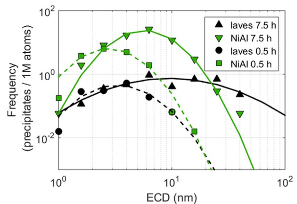
Fig. 8. ECD size frequency histograms for NiAl and Laves phase after 0.5 h and 7.5 h ageing at 540 °C of 9922, determined by APT. The lines represent fits of the data to a lognormal distribution.
