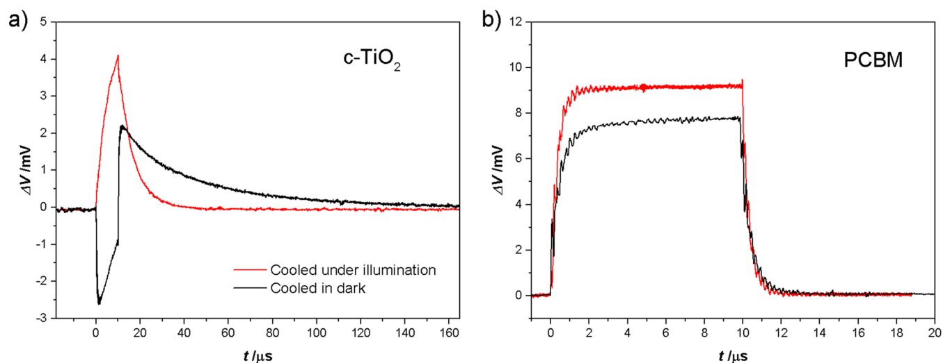
Figure 1. TPV measurements for c\text{-TiO}_2 (a) and PCBM (b) based devices at 223 K cooled under illumination and in the dark. Laser pulse length of 10 \mu\text{s} ; LED bias illumination equivalent to 1 Sun was used.
