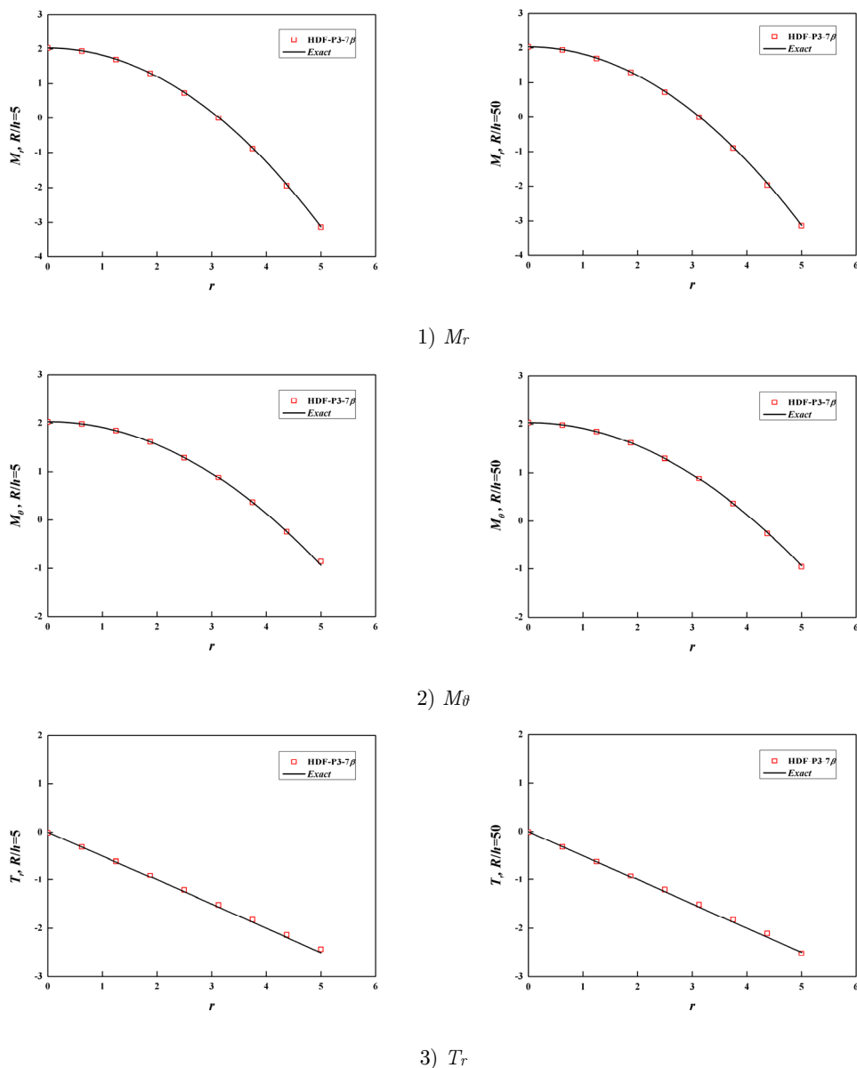
Figure 16: Resultants along the radius of clamped circular plate obtained by the proposed element.
