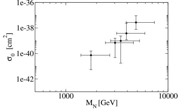
FIG. 51. \sigma_0 [ \text{cm}^2 ] as a function of M_N [GeV]. The results for m_f = 0.030, 0.020, 0.015, 0.012 , and the chiral limit are shown from upper-right to lower-left. Both the statistical and systematic errors are included. The experimentally allowed region is below the plotted window. The current experimental bound for \sigma_0 approximately is 10^{-45}[\text{cm}^2] in this mass range under the assumption that the dark matter interacting in the detector is a thermal relic.
