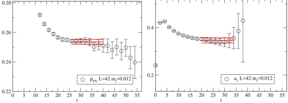
FIG. 6. The effective mass of \rho_{PV} (left) and its staggered parity partner a_1 (right) for N_f = 8 m_f = 0.012 , 42^3 \times 56 .
