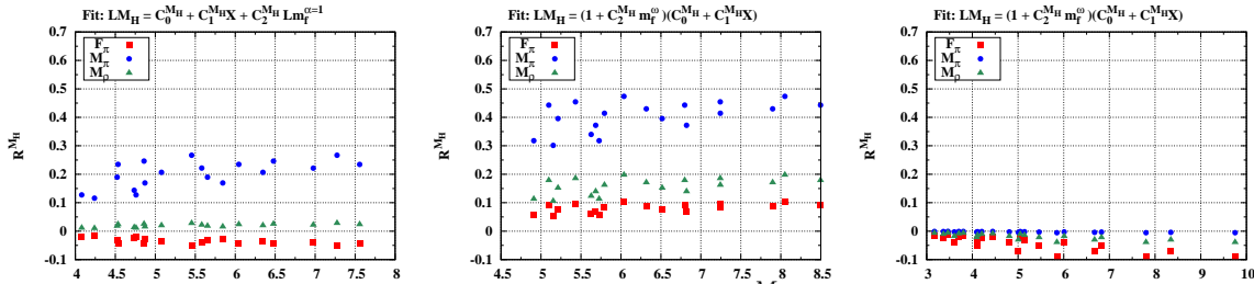
FIG. 39. The strength of the correction term R^{M_H} defined in Eq. (57). Left: In the case of FSHS with power-law correction ( \alpha = 1 ) in N_f = 8 QCD. Middle: In the case of FSHS with RG-motivated correction in N_f = 8 QCD. Right: In the case of FSHS with RG-motivated correction in N_f = 12 QCD with \beta = 3.7 .
