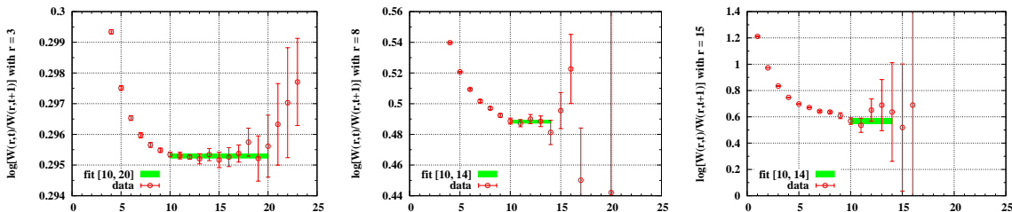
FIG. 40. The Wilson loop potential \mathcal{V}(r, t) given in Eq. (60) for m_f = 0.012 with L = 42 as a function of time t for selected spatial extensions r = 3 (left), 8 (middle), and 15 (right). The green band represents the results of the fit over the plateau.
