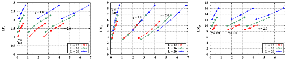
FIG. 36. The FSHS test for N_f = 4 ; the normalized mass spectra LF_\pi (upper left), LM_\pi (upper right), and LM_\rho (lower left) are plotted as a function of the scaling variable X = Lm_f^{1/(1+\gamma)} for selected \gamma .
