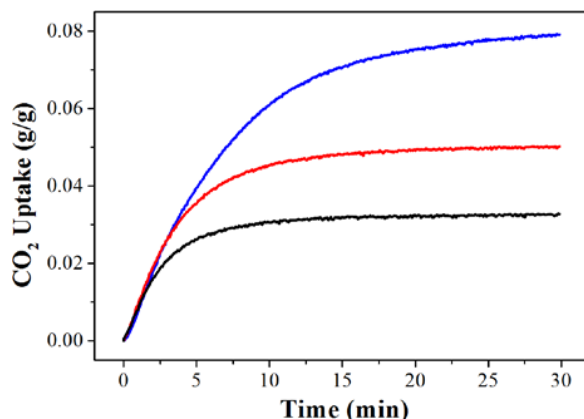
Figure 1. Plot of CO 2 uptake for nitrogen- and sulfur-doped porous carbon (NSPC) as a function of time using pure CO 2 at 1 atm at the temperatures of 24.5, 44.7, and 65.0 °C in blue, red, and black, respectively.
