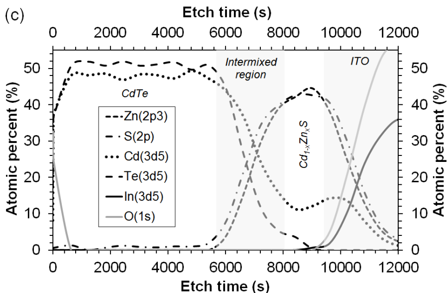
Figure 1: XPS depth profiles for (a) device PZN06, (b) device PZN07 and (c) device PZN14; all having received \text{CdCl}_2 activation treatment.
