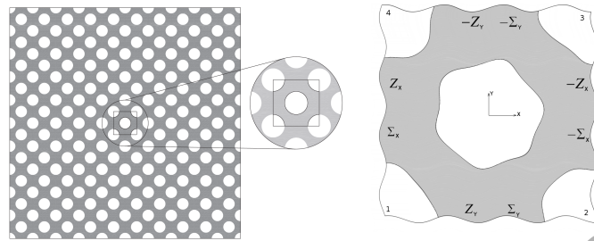
(a) Periodicity: RVE inside an infinite matrix of RVEs. (b) Periodic boundary conditions definition
