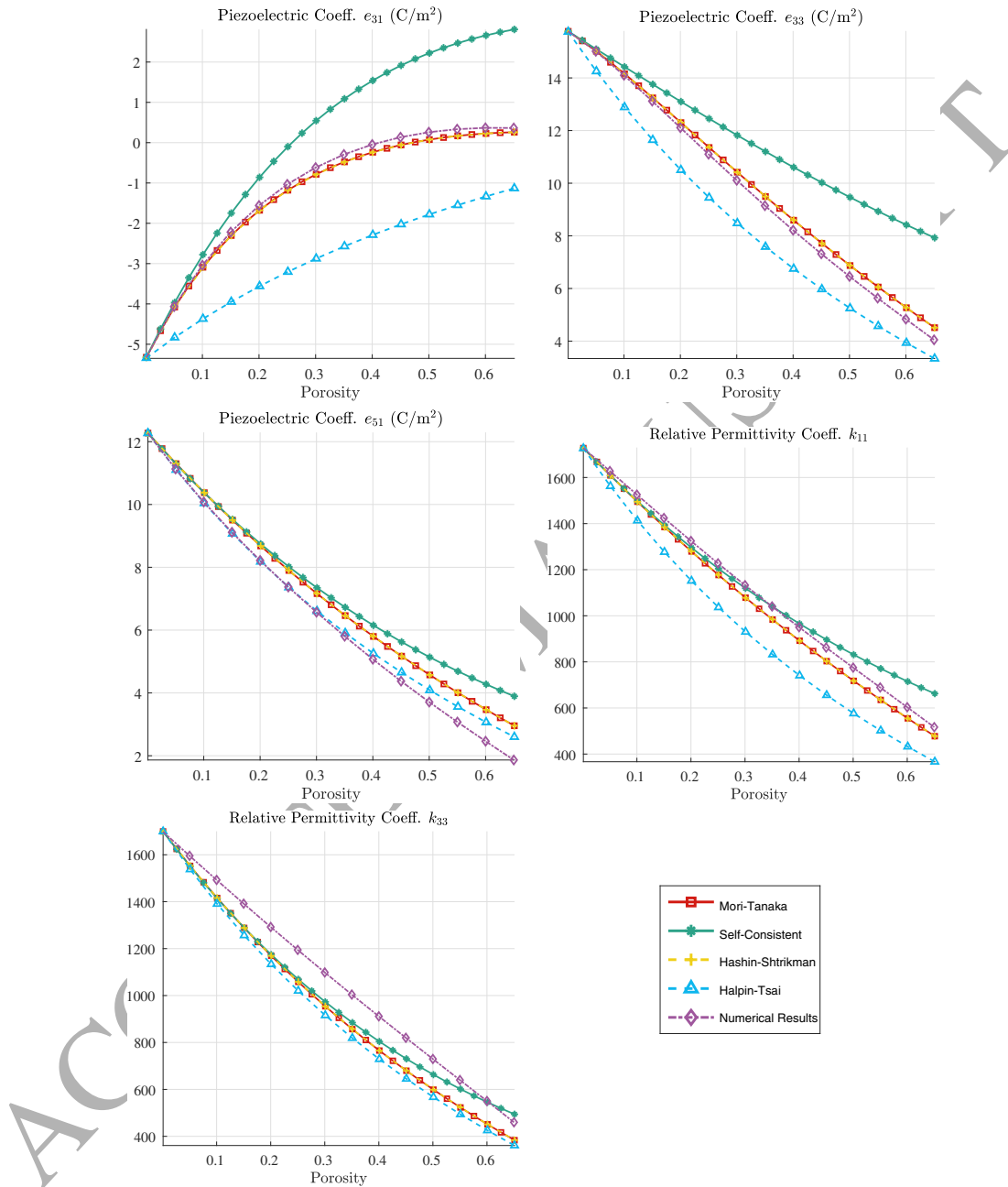
Figure 4: The estimated piezoelectric and dielectric coefficients.
