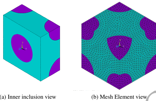
Figure 2: Different views of the representative volume element
