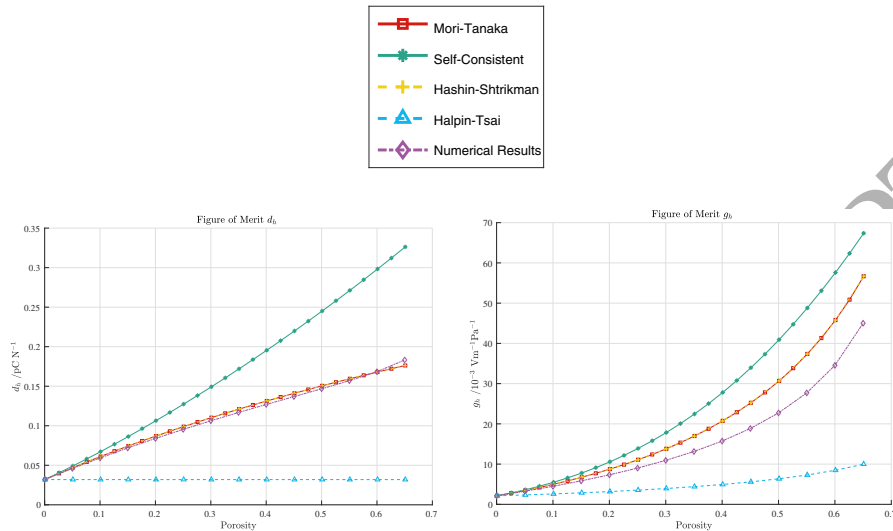
Figure 5: The figures of merit d_h and g_h for the analytical and numerical methods.
