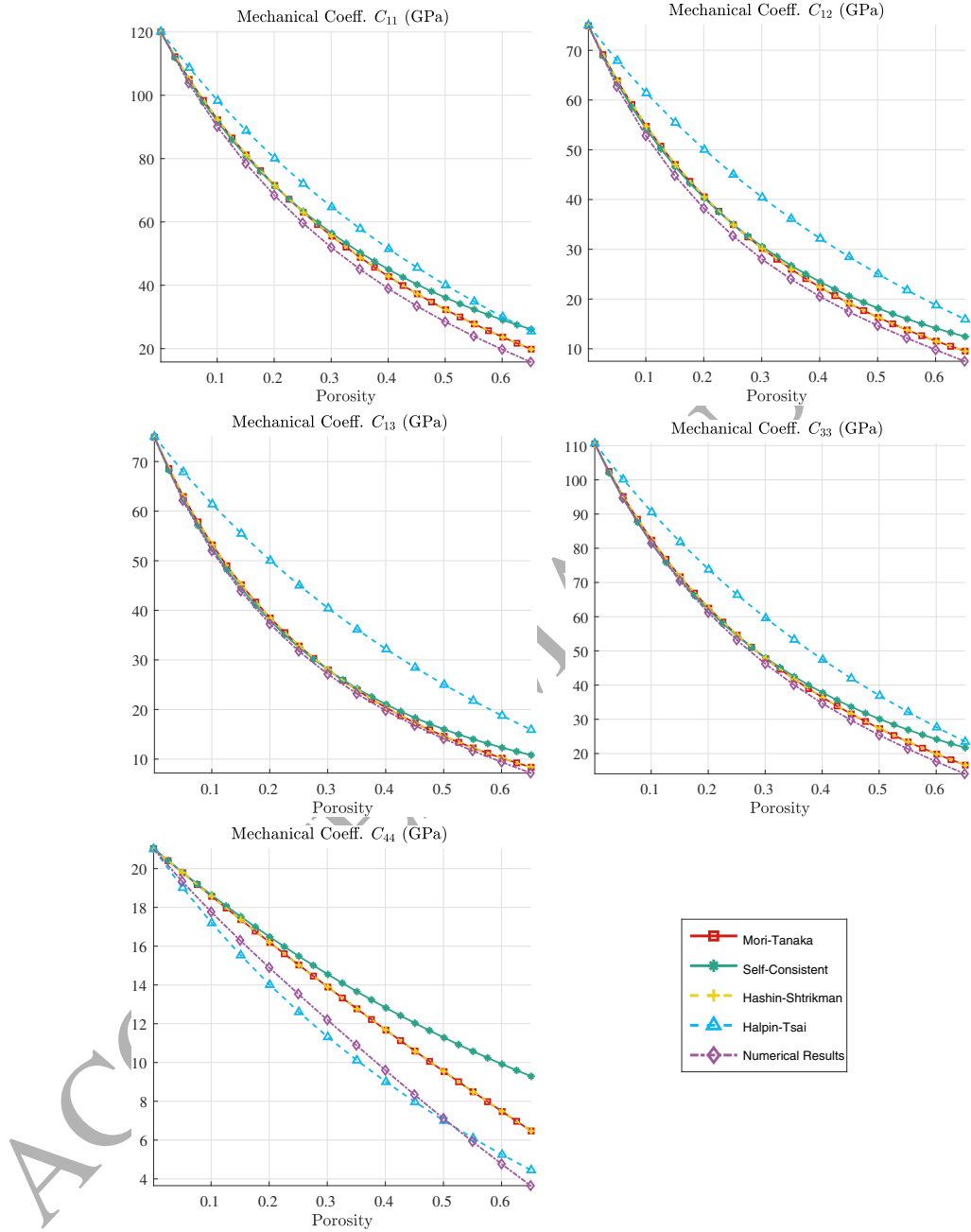
Figure 3: The estimated mechanical coefficients.
