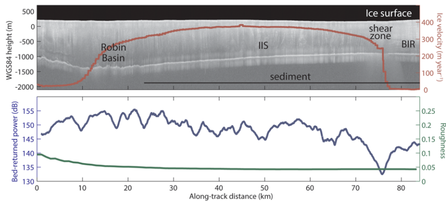
Fig. 4. Radar-sounding profiles, acquired by the British Antarctic Survey in 2010–11, revealing the flat interface indicative of water-saturated basal sediment. Locations for each profile are annotated in Figure 1. IIS, Institute Ice Stream; BIR, Bungenstock Ice Rise. (a) A–A'. (b) B–B'. (c) C–C'. Ice-surface velocities (after Rignot et al. 2011) are provided with bed reflectivities and basal roughness along each profile. Note that in all profiles the association between the greatest ice velocities within the IIS and the region of the bed interpreted as comprising water-saturated basal sediments. Note also in B–B' and C–C' the association between the marked change in ice-surface velocity across the IIS shear margin and the bed reflection strength due a sharp transition between wet (IIS) and frozen (BIR) basal sediments. Taken from Siegert et al. (2016).
