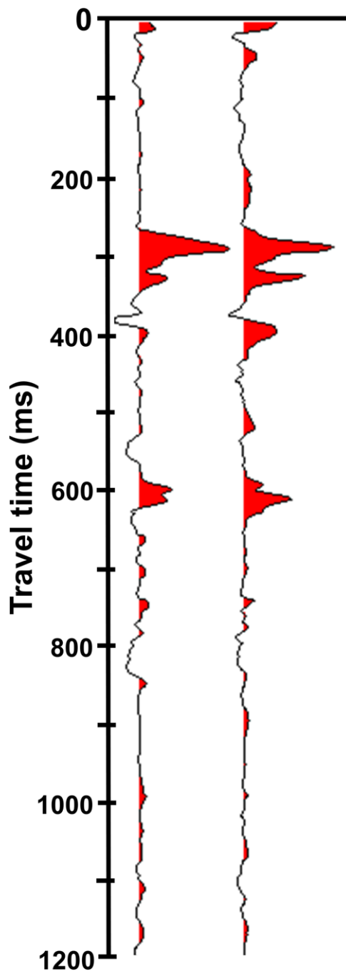
Fig. 6. Representative seismoelectric soundings on the West Greenland Ice Sheet. The two dominant seismoelectric arrivals at c. 305 ms and c. 610 ms were both generated at the ice–bed interface ( c. 1145 \pm 15 m; Booth et al. 2012; Kulesa et al. In review), and are consistent with a seismoelectric conversion and the arrival of co-seismic energy, respectively.
