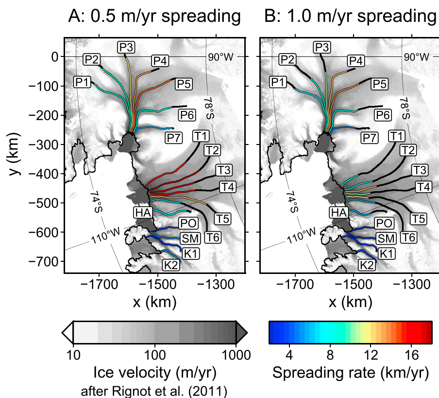
Figure 3. (a) Fitted spreading rates for the 0.5 m/yr threshold value of surface-lowering rates (Figure 2 and Table 1) color coded along the flow lines. The background greyscale shading represents surface ice velocity [Rignot et al. , 2011]. The colored part of the flow lines corresponds to the actual positions to which the respective threshold value has migrated. Black solid extensions indicate the remainders of the flow lines as illustrated in Figure 2 and in the supporting information (270 km at most). (b) The same for the 1.0 m/yr threshold value.
