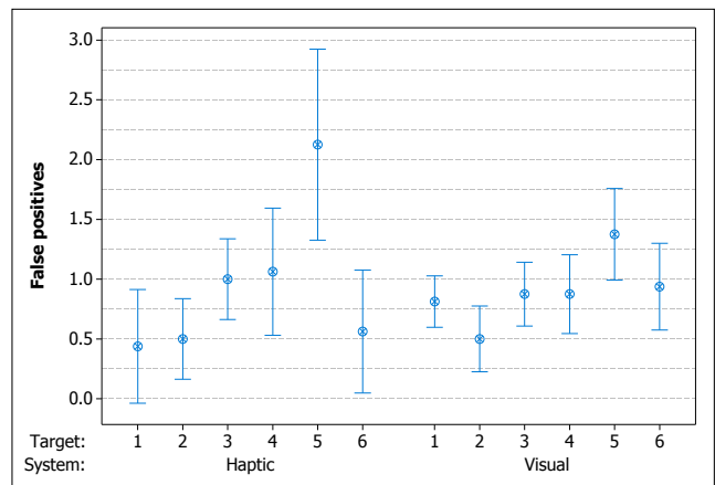
Figure 8: False positives
