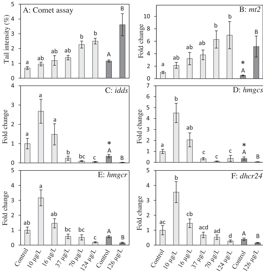
Fig. 1. Effects of copper exposure on F1 Sibilyback and Houghton Spring fish: (A) DNA damage measured using the Comet assay and (B–F) transcript profiling conducted using RT-qPCR. Light-shaded bars represent the Sibilyback population and dark coloured bars represent the population originating from Houghton Springs. Common letters indicate no significant difference (P > 0.05) between groups from the same population. Asterisks indicate a significant difference (P < 0.05) between control groups in each population.
