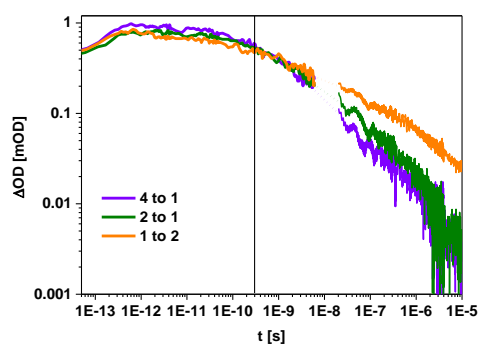
Figure 5. Sub-ps to \mu s transient absorption dynamics of the different blend films, after excitation at 740 nm at 5 \mu\text{J}/\text{cm}^2 and probed at 980 nm, showing similar polaron yields per quenched exciton, but slower recombination as the fullerene concentration is increased.
