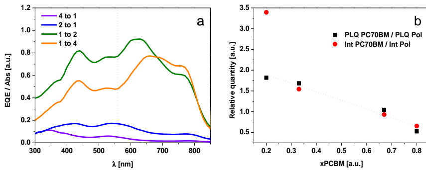
Figure 9. a) EQE/Abs for devices fabricated with 4 to 1, 2 to 1, 1 to 2 and 1 to 4 DPPTT-T:PC 70 BM ratios. The dotted line divides the areas considered for the integration in b), see text. b) PC 70 BM PLQ divided by DPPTT-T PLQ (black squares) and integrated EQE/Abs in the PC 70 BM area (Int PC 70 BM) divided by integrated EQE/Abs in the polymer area (Int Pol) as a function of the fraction amount of PC 70 BM, see text for more details on this relative quantities.
