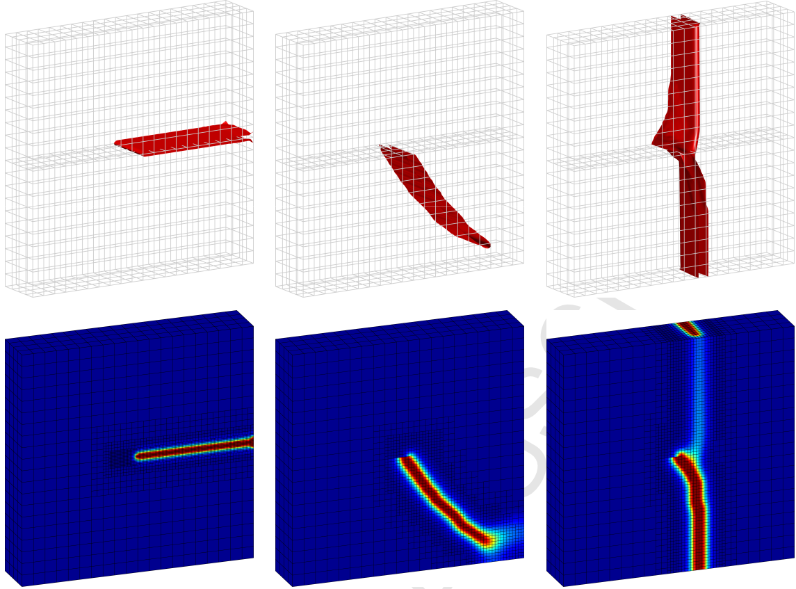
Figure 15: Final phase-field results of mode I (left, for displacement u_z = 0.26 \times 10^{-3} m), mode II (middle, for displacement u_x = 0.37 \times 10^{-3} m) and mode III (right, for displacement u_{y_1} = -u_{y_2} = -1.74 \times 10^{-3} m). Results obtained using the two-field ( \varphi - \mathfrak{s} ) formulation.
