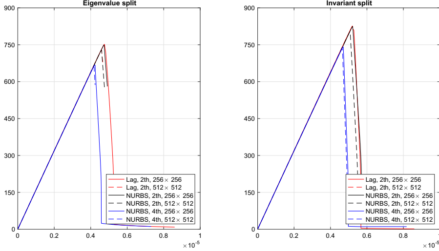
Figure 3: Load-deflection curves for the tension problem using an eigenvalue split (left) and an invariant split (right). Results obtained with the two-field ( \varphi - \mathfrak{s} ) formulation.
