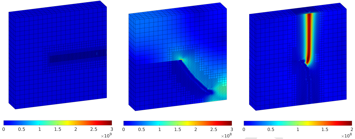
Figure 14: Von Mises stress results of mode I (left, for displacement u_z = 0.26 \times 10^{-3}\text{m} ), mode II (middle, for displacement u_x = 0.37 \times 10^{-3}\text{m} ) and mode III (right, for displacement u_{y1} = -u_{y2} = -1.74 \times 10^{-3}\text{m} ). Results obtained using the two-field (\varphi - \mathfrak{s}) formulation
