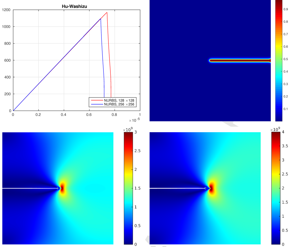
Figure 6: Tension problem, upper row: Load-deflection curve for the tension problem and phase-field results for the fully broken state. Results obtained with the Hu-Washizu mixed variational formulation. Lower Row: von Mises stress distribution at the crack tip. Left: Two-field ( \varphi - \mathfrak{s} ) formulation, right: Hu-Washizu mixed variational formulation. Note the different colorbar ranges.
