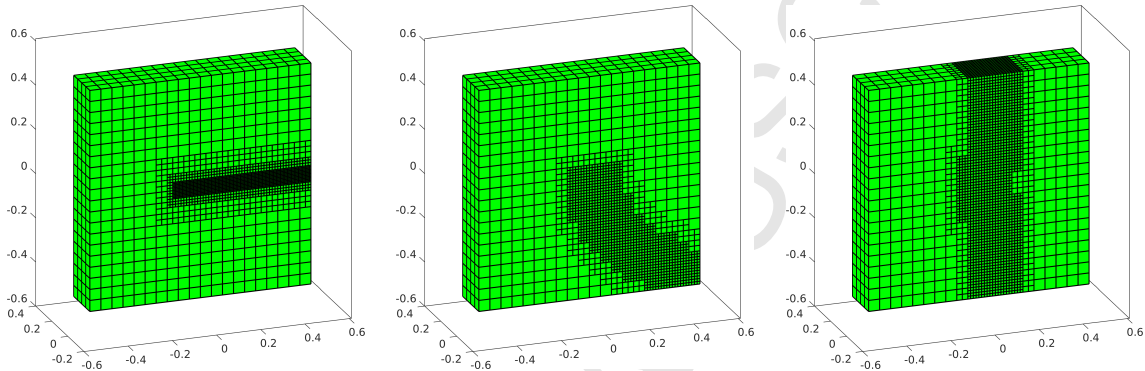
Figure 13: Initial meshes of mode I (left), mode II (middle) and mode III (right)
