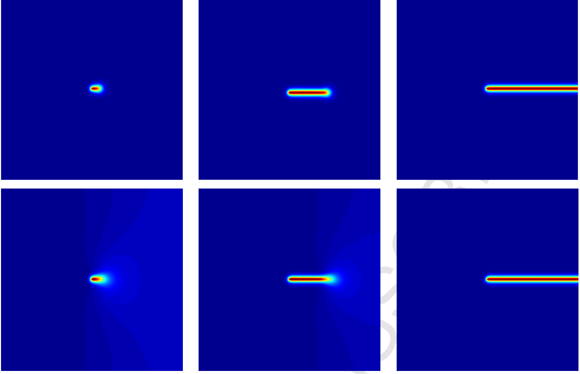
Figure 2: Tension problem: Phase-field results for displacements of u_y = [4.73, 4.83, 4.98] \times 10^{-6} m using the cubic degradation function with a_g = 0.1 (upper row) and for displacements of u_y = [4.47, 4.69, 4.83] \times 10^{-6} m using the quadratic degradation function (lower row). Results for the Neo-Hookean model with anisotropic split of the invariants are presented. Results obtained with the two-field ( \varphi - \mathfrak{s} ) formulation.
