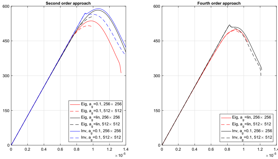
Figure 9: Load-deflection curves for the shear problem for the second and the fourth order regularisation profile. Results obtained with the two-field (\varphi - \mathfrak{s}) formulation.
