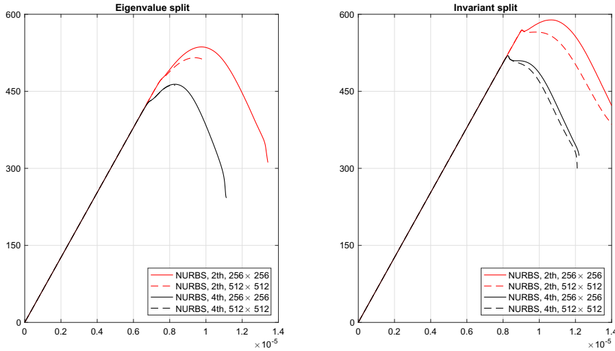
Figure 8: Load-deflection curves for the shear problem for the different splits using an eigenvalue and a decomposition of the invariants. Results obtained with the two-field ( \varphi - \mathfrak{s} ) formulation.
