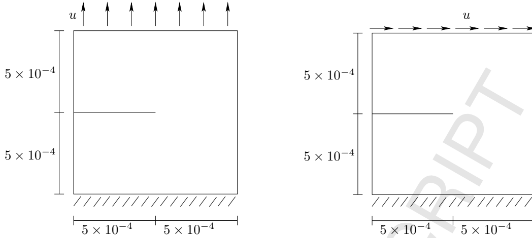
Figure 1: Geometry and boundary conditions for the tension problem (left) and the shear problem (right).
