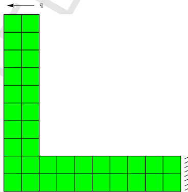
Figure 10: Reference configuration of the large deformation test. A coarse mesh is displayed for visualisation purposes.
