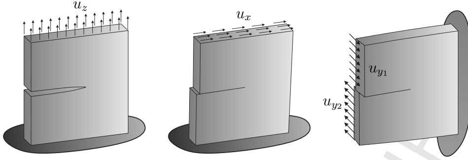
Figure 12: Boundary conditions for mode I (left), mode II (middle) and mode III (right) crack propagation.
