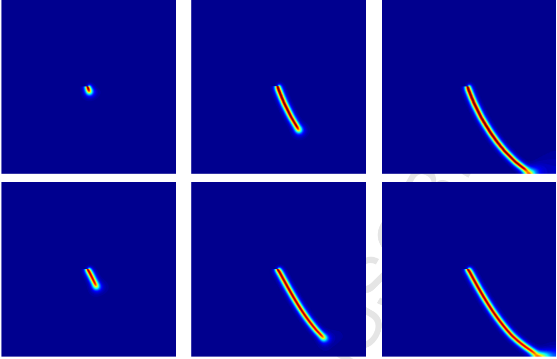
Figure 7: Shear problem: Phase-field results for displacements of u_x = [8.5, 10.5, 1.22] \times 10^{-6} m using the Neo-Hookean model with an anisotropic split of the principal invariants (upper row) and for displacements of u_x = [8.5, 10.5, 11.05] \times 10^{-6} m using the Neo-Hookean model with an anisotropic split of the principal eigenvalues (lower row). In both a parameter of a_g = 0.1 is used for the cubic degradation function. Results obtained with the two-field (\varphi - \mathfrak{s}) formulation.
