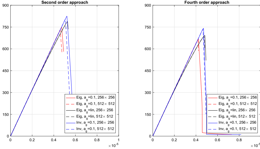
Figure 4: Load-deflection curves for the tension problem for the second and the fourth order regularisation profile. Results obtained with the two-field ( \varphi - \mathfrak{s} ) formulation.
