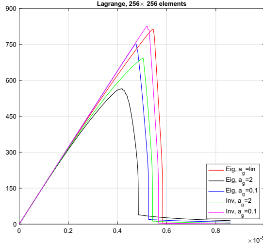
Figure 5: Load-deflection curves for the tension problem. Study of different a_g parameters for the cubic degeneration function. Results obtained with the two-field (\varphi - \mathfrak{s}) formulation.
