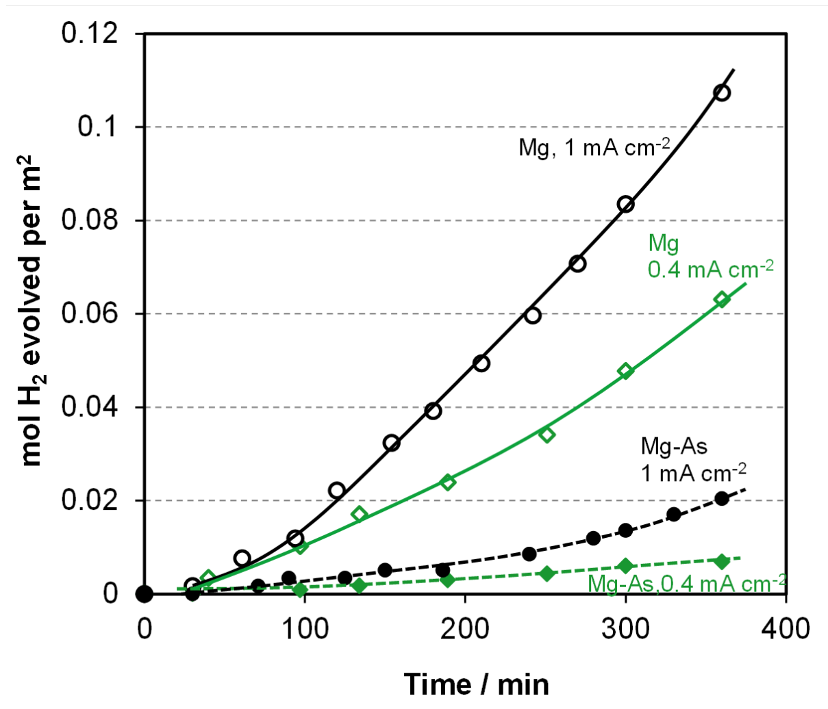
Figure 11: Plots of moles hydrogen gas evolved versus time for Mg and Mg-As (0.37%) under galvanostatic polarisation in 0.1 \text{ mol dm}^{-3} NaCl at pH 7.
