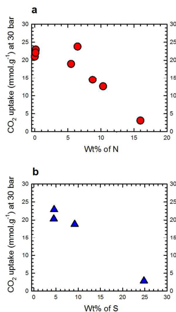
Fig. 13 High pressure (30 bar) CO 2 uptake as a function of (a) N wt% and (b) S wt% in NPC and SPC samples, respectively. Sorption measurements were performed at 24 °C.
