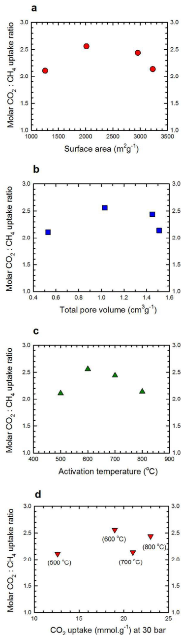
Fig. 19 Plot of molar CO 2 :CH 4 uptake ratio (@ 30 bar) as a function of the (a) surface area, (b) total pore volume, (c) activation temperature, and (d) CO 2 uptake for PPy-T-2 ( T = 500, 600, 700 and 800 °C) NPC samples. Sorption measurements were performed at 24 °C.
