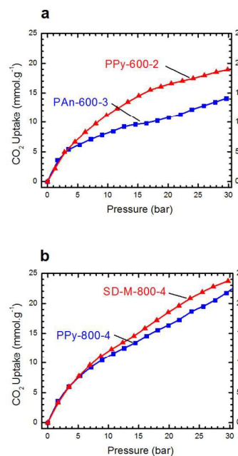
Fig. 14 High pressure CO 2 adsorption uptake for (a) PAN-600-3 compared with PPy-600-2 and (b) SD-M-800-4 compared with PPy-800-4. Sorption measurements were performed at 24 °C.
