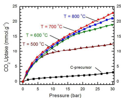
Fig. 1 CO 2 uptake as a function of CO 2 pressure on activated PPy-T-2 in comparison with the PPy precursor. Sorption measurements were performed at 24 °C.
