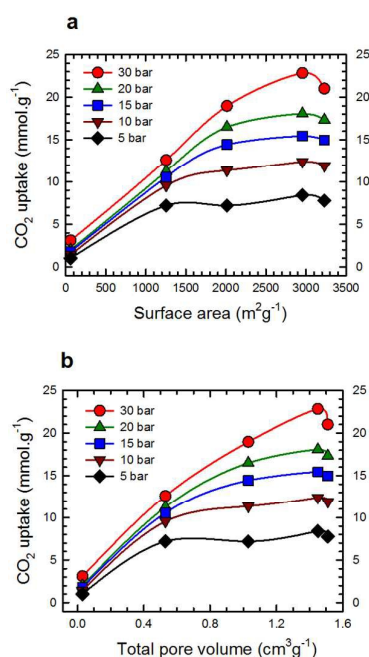
Fig. 4 Dependence of CO 2 uptake on (a) surface area and (b) total pore volume. PC samples were synthesized from polypyrrole and activated by KOH each at a different fixed temperature. Solid lines are only to guide the eye. Sorption measurements were performed at 24 °C.
