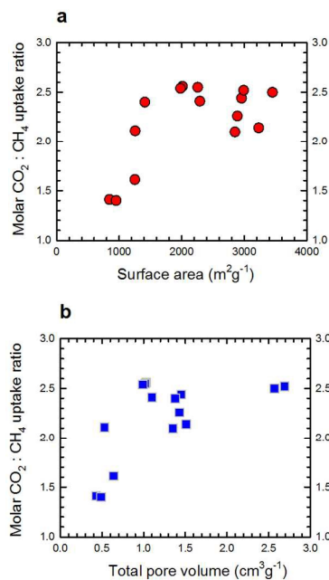
Fig. 18 Plot of molar CO 2 :CH 4 uptake ratio (@ 30 bar) as a function of the (a) surface area and (b) total pore volume, for a range of PC, NPC and SPC samples. Sorption measurements were performed at 24 °C.
