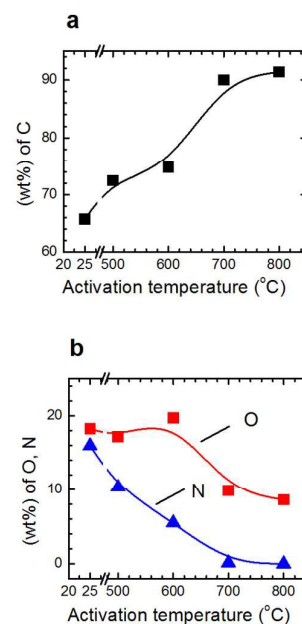
Fig. 12 The wt% determined by XPS of elemental (a) carbon and (b) oxygen and nitrogen versus activation temperature for the PPy precursor and PPy-T-2 samples.
