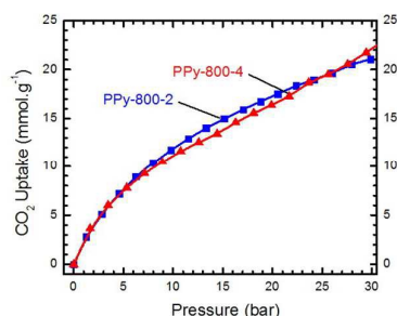
Fig. 10 High pressure volumetric \text{CO}_2 adsorption uptake measurements on PPy-800-2 and PPy-800-4 showing the effect of the KOH:precursor ratio. Sorption measurements were performed at 24^\circ\text{C} .
