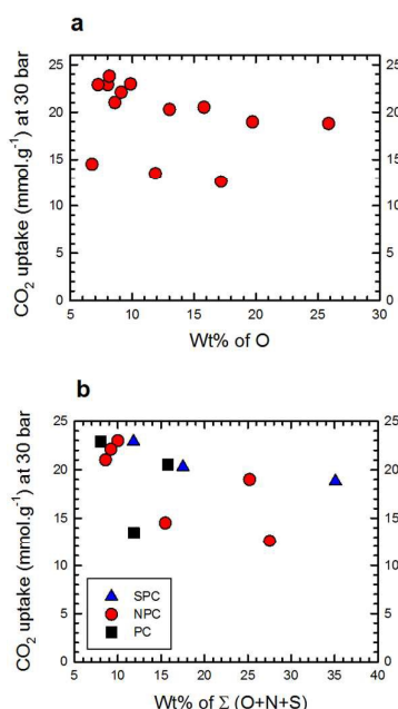
Fig. 16 The high pressure (30 bar) CO 2 uptake as a function of (a) O wt% and (b) Σ(O,N,S) wt% in PC, NPC and SPC samples. Sorption measurements were performed at 24 °C.
