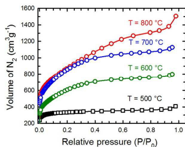
Fig. 2 N 2 adsorption isotherms for four different NPC samples PPy-T-2 prepared from polypyrrole and activated at the labelled temperature (T). Sorption measurements were performed at 24 °C.
