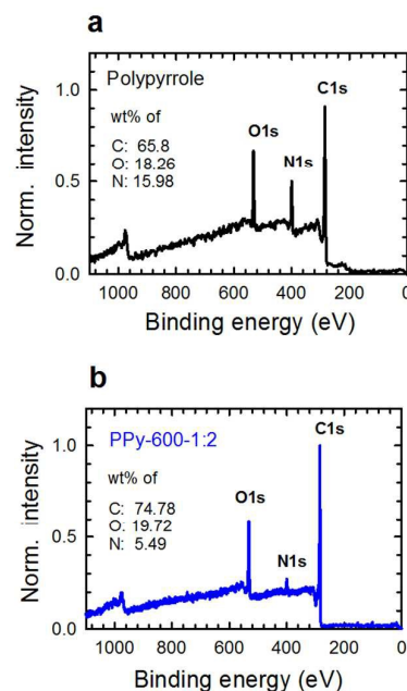
Fig. 11 Typical XPS survey scans for (a) the polypyrrole precursor and (b) PPy-600-2 NPC samples.
