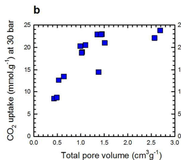
Fig. 3 High pressure CO 2 uptake (@ 30 bar and 24 °C) as a function of the (a) surface area and (b) total pore volume, for a range of PC, NPC and SPC samples.
