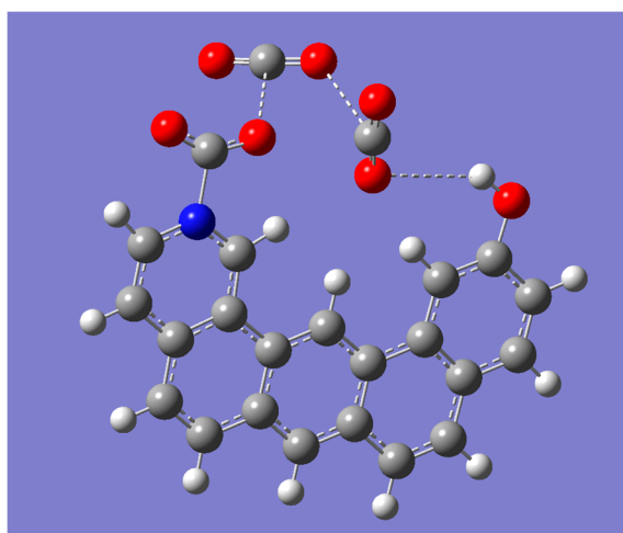
Figure 9. Optimized energy minimum structure for the interaction of the model Lewis acid/base functionalized dibenzo[ a,j ]anthracene (Figure 8) with CO 2 . Selected bond lengths and angles: N···C = 1.633 Å, H···O = 2.994 Å, C···O = 2.545 and 2.729 Å, O–C–O = 140.1°, 175.3° and 173.8°.
