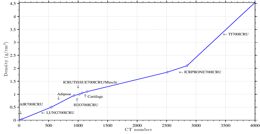
Fig. 3: The CT ramp for the conversion of CT values to material type and densities used in OMP. The same ramp was used in MC, the density and composition of the material used in this ramp were included in the PEGS4 cross section data file.
