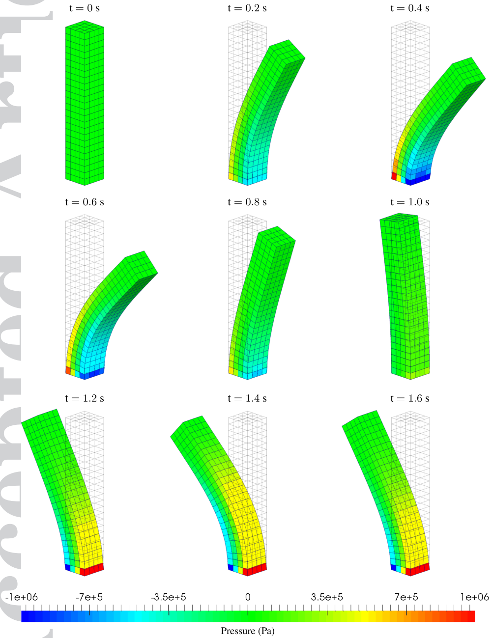
Figure 22. Bending column configuration
