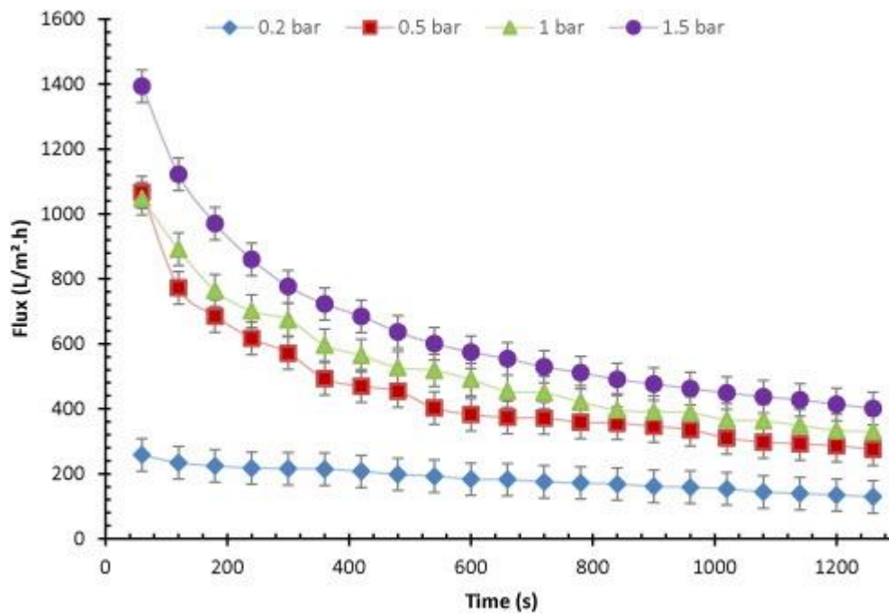
Fig. 6. Flux versus filtration time at different operating pressures during MF of the resin suspension with 0.1 μm PVDF membrane. The resin concentration is 1.0 g/L, pH = 6, and T = 25 °C.
