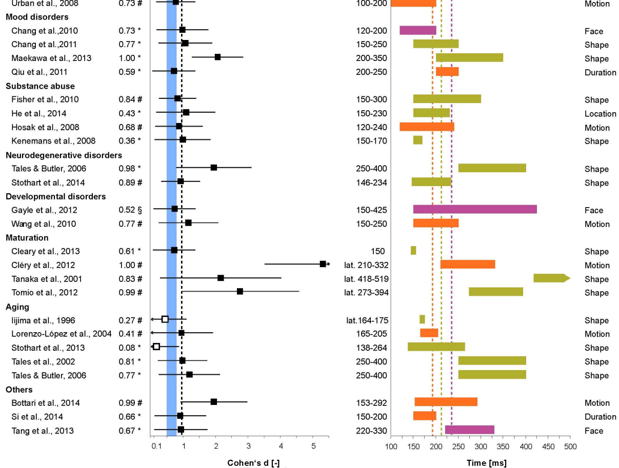
Fig. 7. Equivalent effect size, study power, interval of difference and type of stimulation among selected studies (see Effect size and power of the vMMN studies ). Forest plot in the left panel shows the estimate of equivalent Cohen's effect size (black squares for significant and opened squares for not significant observations), horizontal black lines represent 95 percentile intervals. Cohen's d was computed from the f value (marked as *), from the p value (#), or from correlation coefficient (§), as it is marked in the column Power . The power was calculated from the eCd and group size. The blue bar marks the interval of Cohen's d for a medium effect size (0.5 – 0.8). The dotted line delineates the eCd median. Forest plot in the right panel shows intervals of the vMMN difference between groups. The Interval column lists intervals in milliseconds for amplitude evaluation. In case when latency was assessed, the lat precedes the indicated interval of intergroup means. In the right side column Domain lists stimulus types used in the studies. The green bars mark a task with a spatial encoding of deviancy, and the orange ones represent the deviancy encoded by a temporal stimulus aspect.
