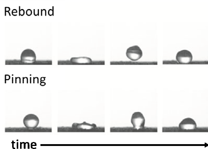
Figure 2. Images, taken from a high speed video recording, show the difference between rebound and pinning behaviour of a droplet impacting on a fixed, particulate surface.
