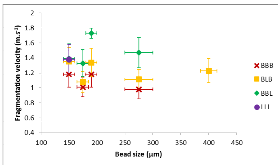
Figure 8. A graph showing the fragmentation velocities of the bead pack against bead size. Legend describes base layer to top layer and whether the layer is hydrophobic (B) or hydrophilic (L). Error in bead size due to difference in sieve sizes, velocity error due to measurement errors.
