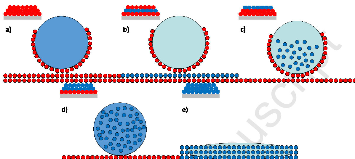
Figure 9. Diagram showing bead behaviour after droplet impact for each bead pack configuration. Schematic of bead pack shown at the top, indicating which layers are hydrophobic (red) or hydrophilic (blue).
