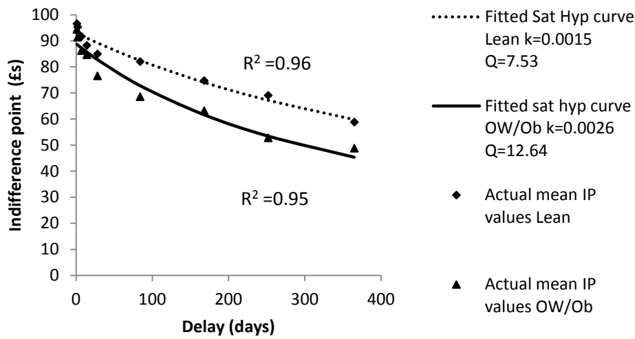
Figure 2: Graph to show the Q and satk values and saturating-hyperbolic curves fitted to the mean indifference points for lean and overweight/obese (OW/Ob) participants (N=79).
