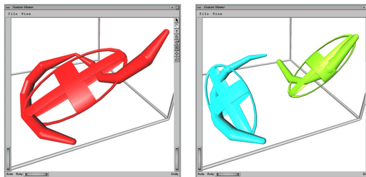
Figure 23: A split event, before (left) and after (right). The features are visualised with both an ellipsoid and a skeleton icon 31 .
