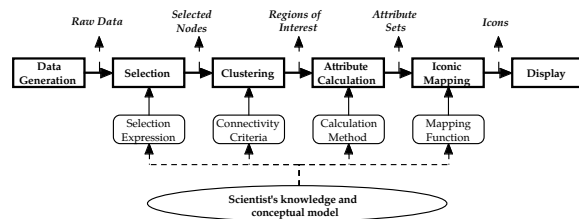
Figure 2: The feature extraction pipeline 36 .
