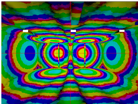
Figure 10: Phase visualization of sound received at one listener position for the first reflection. [BMD*08]. Image courtesy of
