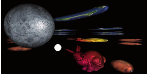
Figure 12: Multiply appearing objects and a point light source in the Gödel's universe [GMDW09].
